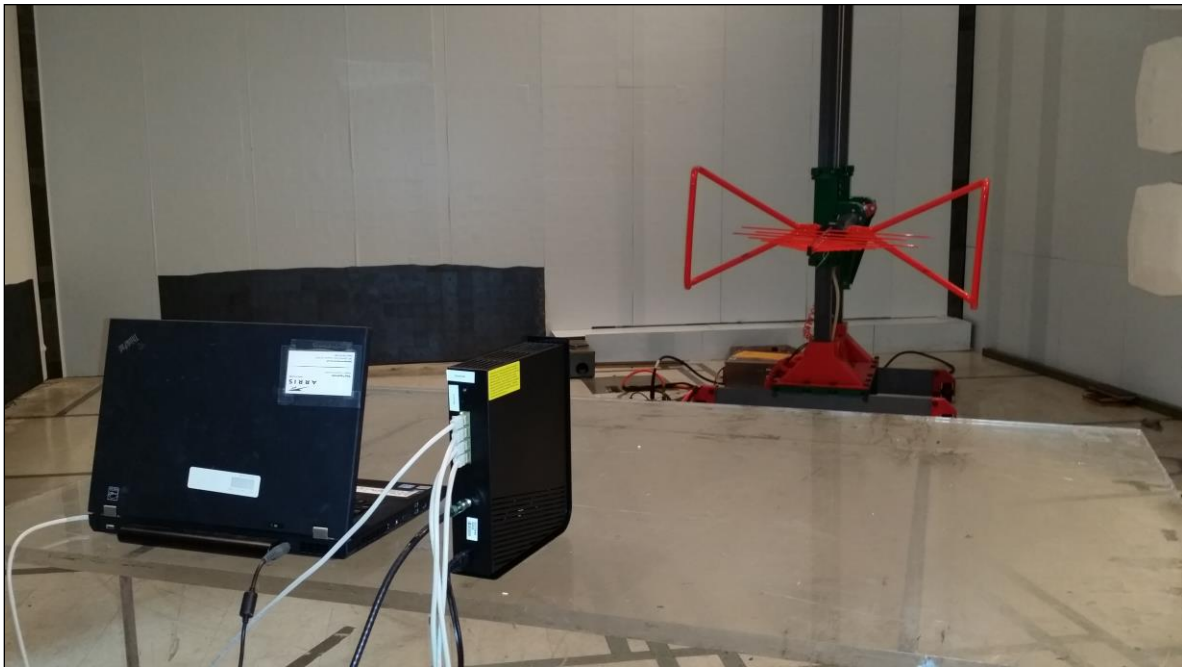
Photograph 2. Radiated Emission, Test Setup, 30 MHz – 1 GHz
