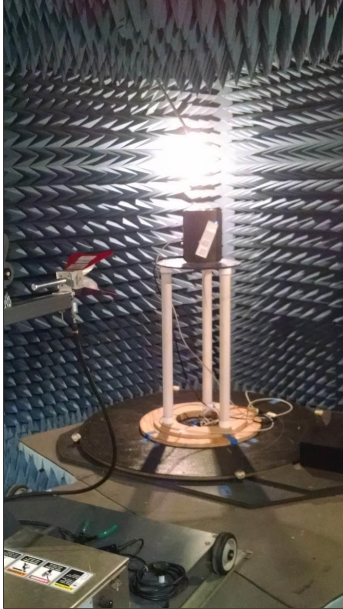
Photograph 2. Radiated Test Setup, 1 GHz – 18 GHz
