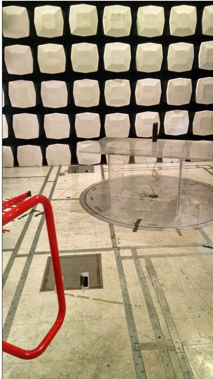
Photograph 1. Radiated Test Setup, 30 MHz – 1 GHz
