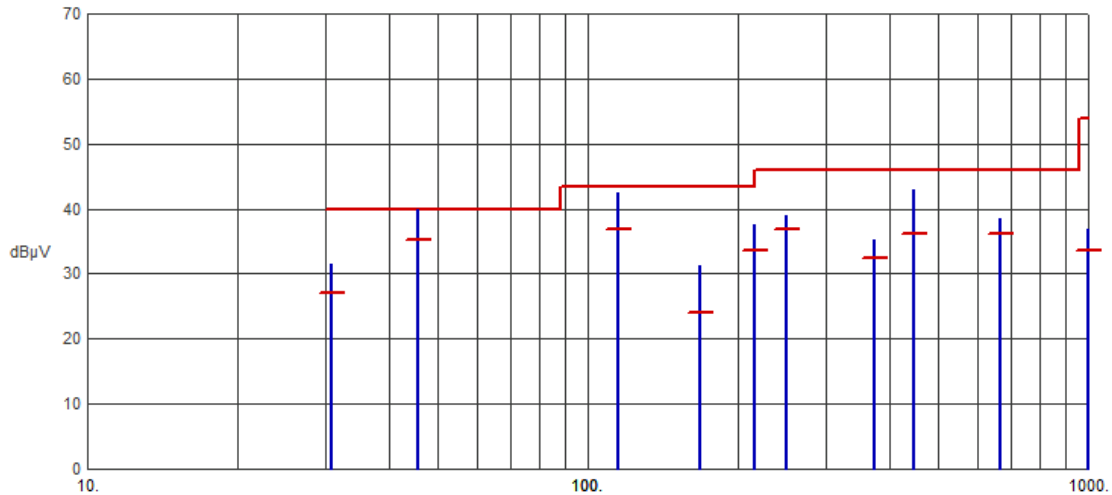
Test No.: 219-13, Radiated Emissions - Vertical Polarity
