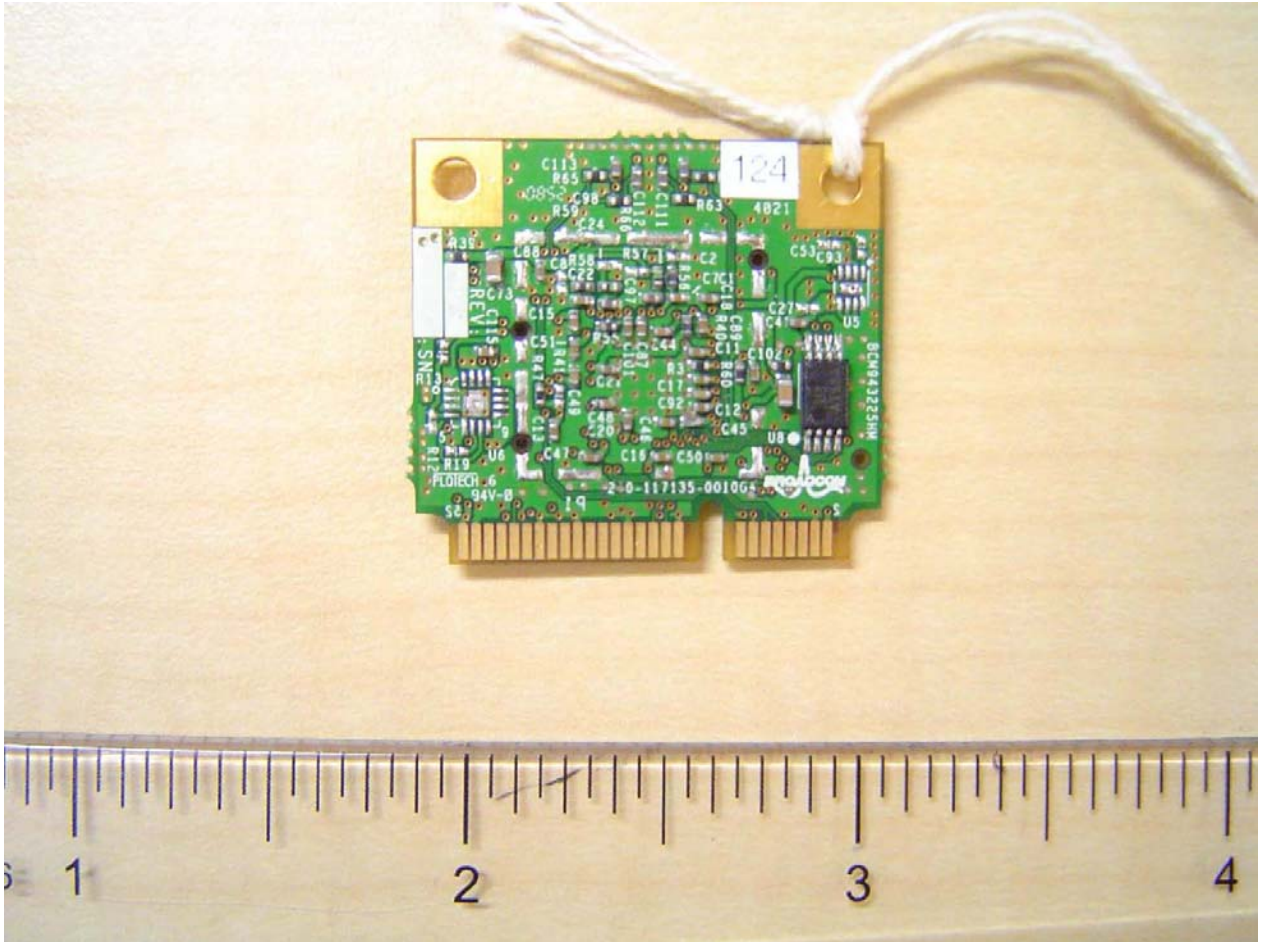
Figure 2: PCB - Back
