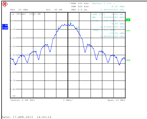
Figure 7.3.2-9: 6dB Bandwidth – 2480 MHz - ANT 1
