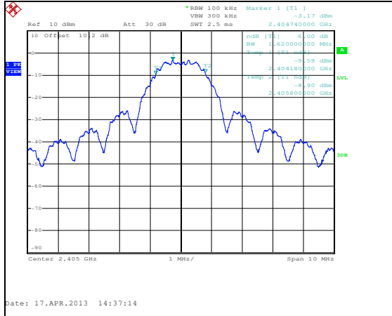
Figure 7.3.2-7: 6dB Bandwidth – 2405 MHz - ANT 1
