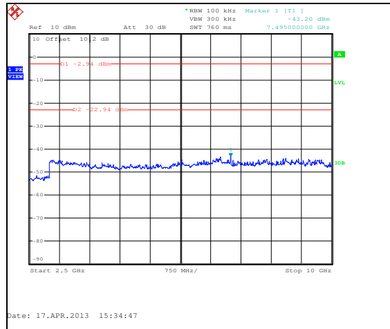
Figure 7.5.1.2-8: 2.5 GHz – 10 GHz – 2480 MHz – ANT 0
