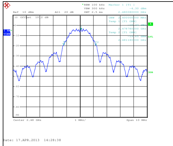
Figure 7.3.2-6: 99% Bandwidth – 2480 MHz – ANT 0
