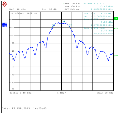
Figure 7.3.2-3: 6dB Bandwidth – 2480 MHz – ANT 0
