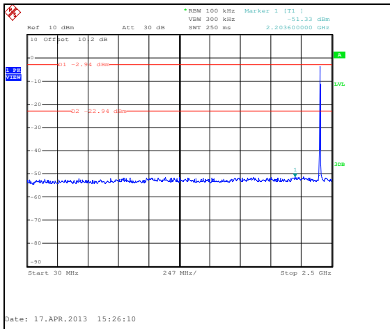
Figure 7.5.1.2-1: 30 MHz – 2.5 GHz – 2405 MHz – ANT 0
