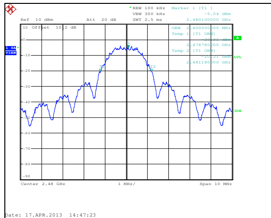
Figure 7.3.2-12: 99% Bandwidth – 2480 MHz - ANT 1
