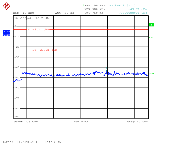
Figure 7.5.1.2-19: 2.5 GHz – 10 GHz – 2480 MHz – ANT 1
