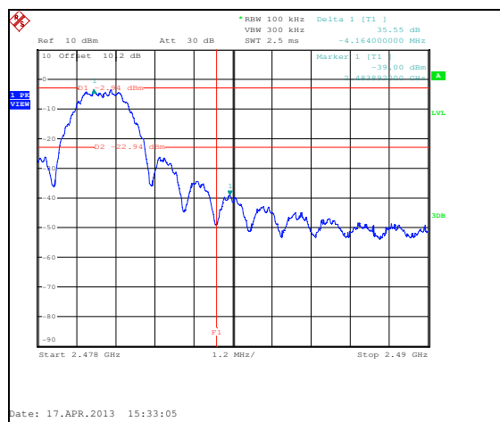
Figure 7.5.1.2-11: Upper Band-edge - 2480 MHz – ANT 0
