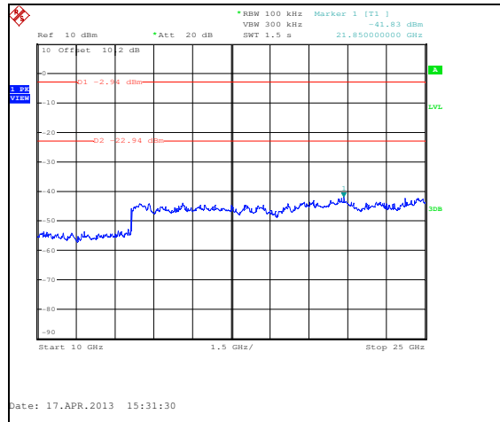
Figure 7.5.1.2-6: 10 GHz – 25 GHz – 2440 MHz – ANT 0
