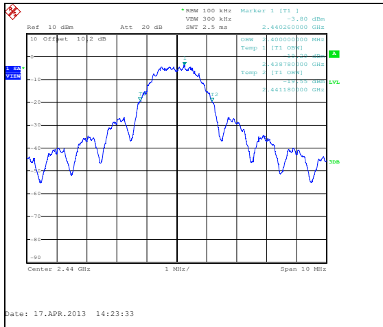
Figure 7.3.2-5: 99% Bandwidth – 2440 MHz – ANT 0
