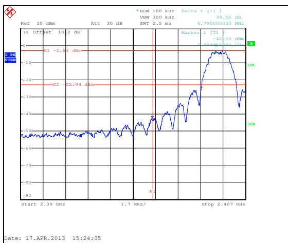
Figure 7.5.1.2-10: Lower Band-edge - 2405 MHz – ANT 0
