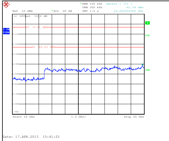
Figure 7.5.1.2-14: 10 GHz – 25 GHz – 2405 MHz – ANT 1
