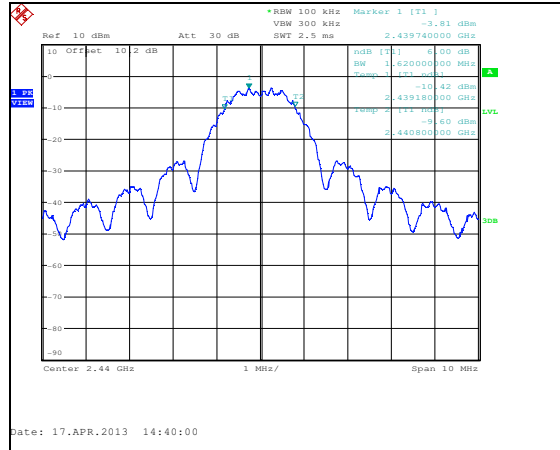
Figure 7.3.2-8: 6dB Bandwidth – 2440 MHz - ANT 1
