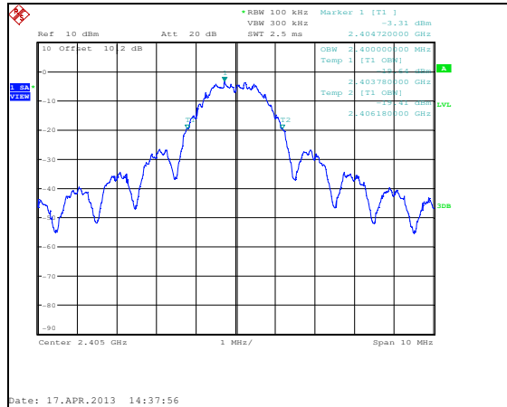
Figure 7.3.2-10: 99% Bandwidth – 2405 MHz - ANT 1
