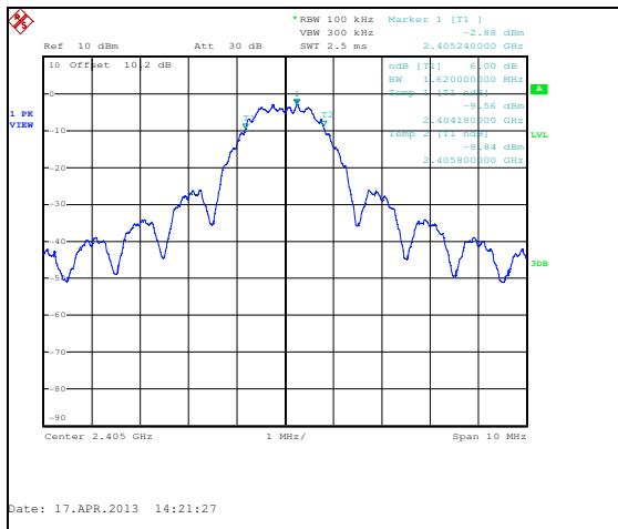
Figure 7.3.2-1: 6dB Bandwidth – 2405 MHz - ANT 0
