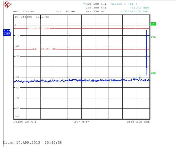
Figure 7.5.1.2-15: 30 MHz – 2.5 GHz – 2440 MHz – ANT 1
