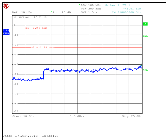
Figure 7.5.1.2-9: 10 GHz – 25 GHz – 2480 MHz – ANT 0
