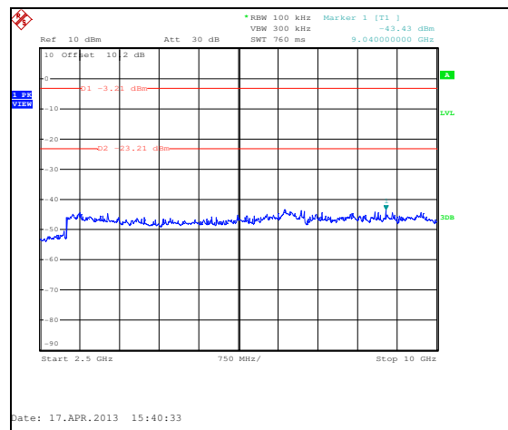
Figure 7.5.1.2-13: 2.5 GHz – 10 GHz – 2405 MHz – ANT 1
