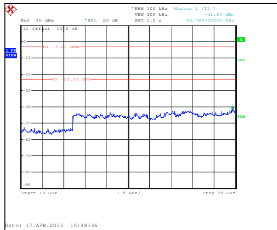
Figure 7.5.1.2-17: 10 GHz – 25 GHz – 2440 MHz – ANT 1
