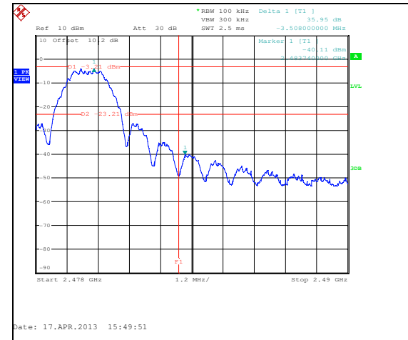
Figure 7.5.1.2-22: Upper Band-edge - 2480 MHz – ANT 1
