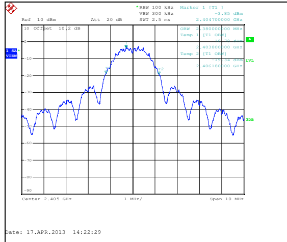
Figure 7.3.2-4: 99% Bandwidth – 2405 MHz – ANT 0
