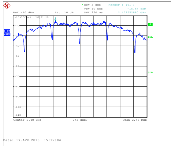
Figure 7.6.2-6: PSD Plot – 2480 MHz
