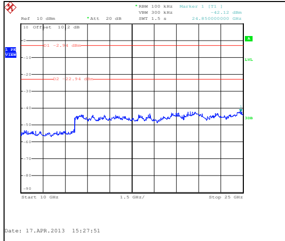
Figure 7.5.1.2-3: 10 GHz – 25 GHz – 2405 MHz – ANT 0
