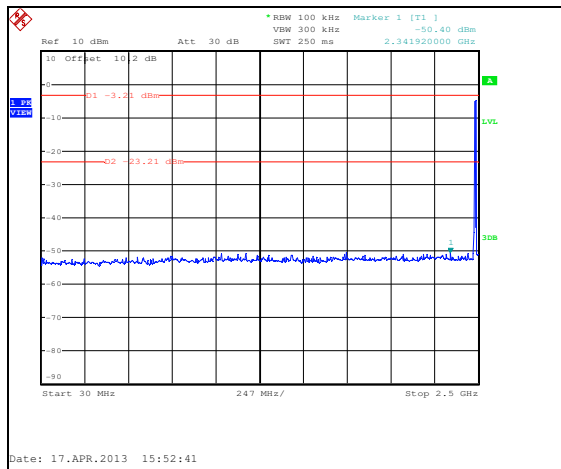
Figure 7.5.1.2-18: 30 MHz – 2.5 GHz – 2480 MHz – ANT 1
