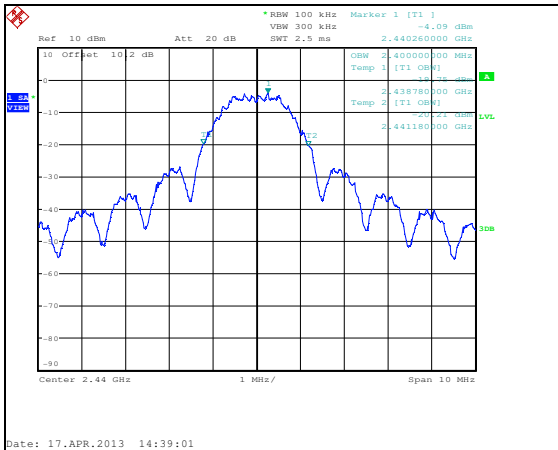
Figure 7.3.2-11: 99% Bandwidth – 2440 MHz - ANT 1
