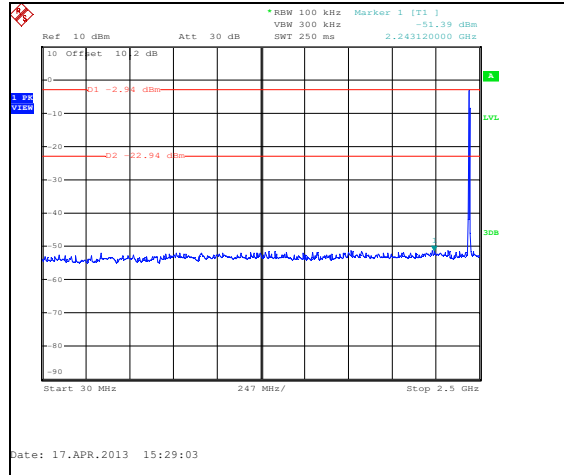
Figure 7.5.1.2-4: 30 MHz – 2.5 GHz – 2440 MHz – ANT 0
