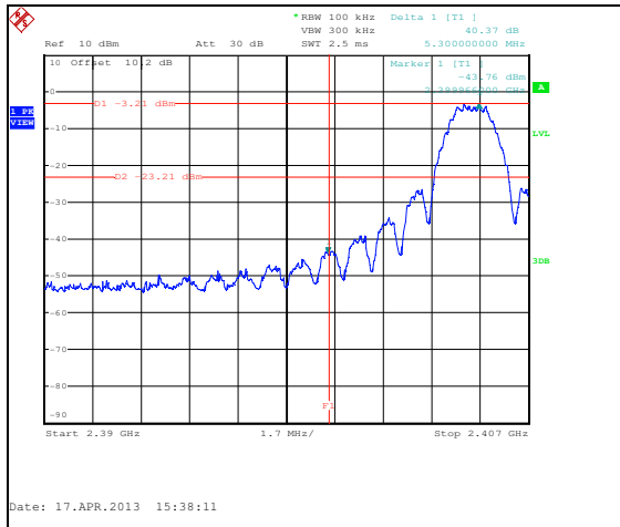
Figure 7.5.1.2-21: Lower Band-edge - 2405 MHz – ANT 1
