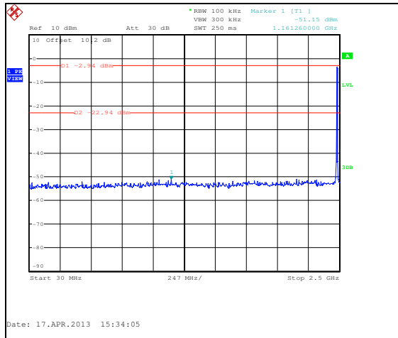
Figure 7.5.1.2-7: 30 MHz – 2.5 GHz – 2480 MHz – ANT 0
