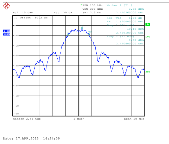
Figure 7.3.2-2: 6dB Bandwidth – 2440 MHz - ANT 0
