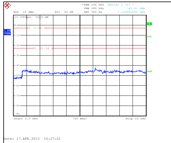
Figure 7.5.1.2-2: 2.5 GHz – 10 GHz – 2405 MHz – ANT 0
