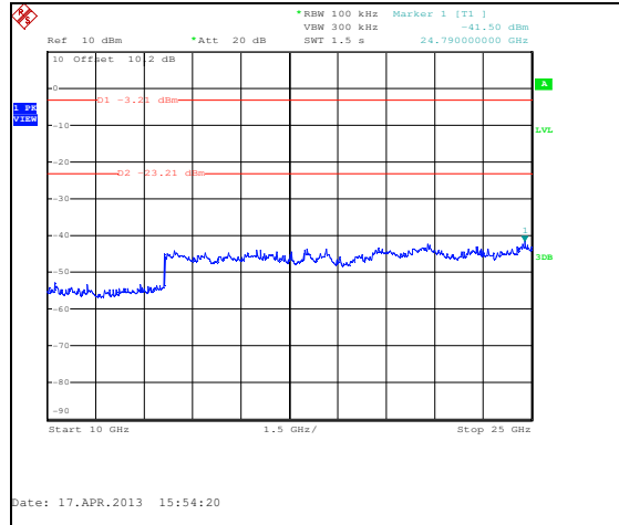
Figure 7.5.1.2-20: 10 GHz – 25 GHz – 2480 MHz – ANT 1
