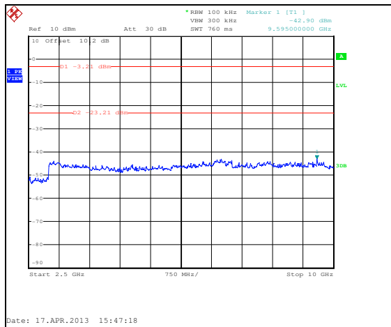
Figure 7.5.1.2-16: 2.5 GHz – 10 GHz – 2440 MHz – ANT 1
