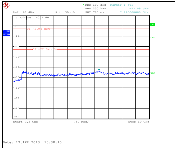
Figure 7.5.1.2-5: 2.5 GHz – 10 GHz – 2440 MHz – ANT 0
