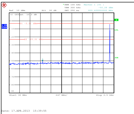
Figure 7.5.1.2-12: 30 MHz – 2.5 GHz – 2405 MHz – ANT 1
