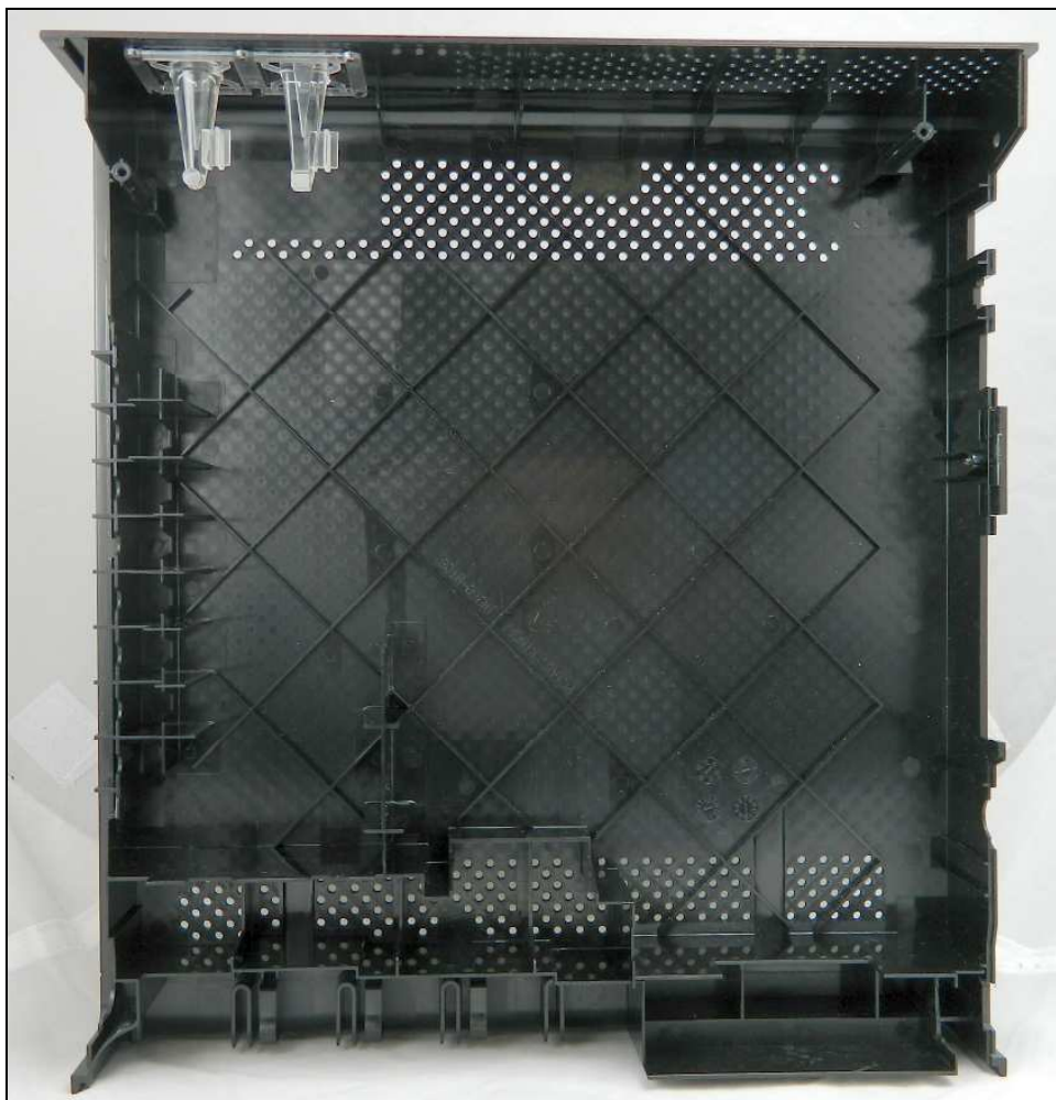
Figure 2: Internal Photo
