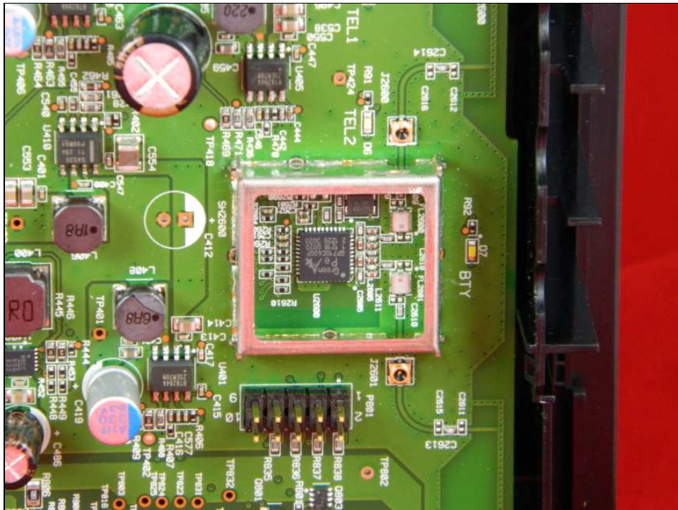
Figure 9: Internal Photo Zigbee (Shields Removed)
