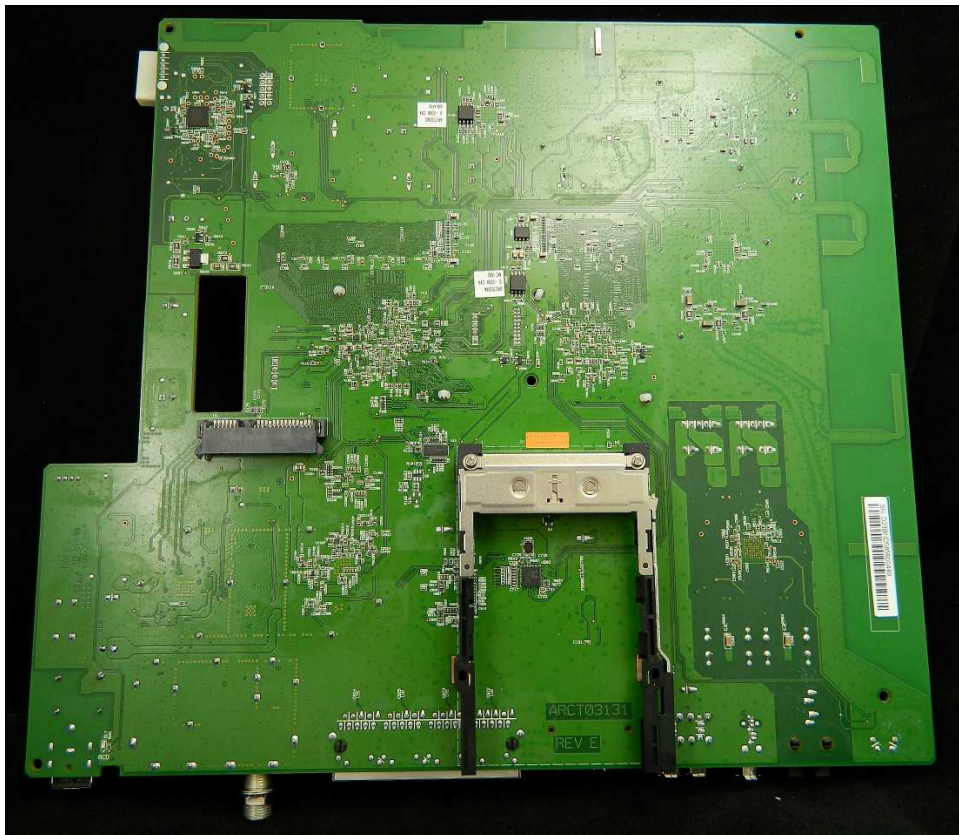
Figure 11: Internal Photo
