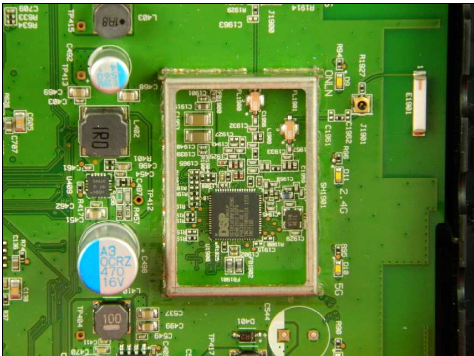
Figure 8: Internal Photo DECT (Shields Removed)
