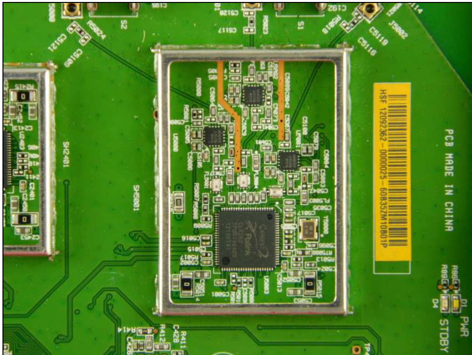
Figure 7: Internal Photo 802.11 a/n (Shields Removed)
