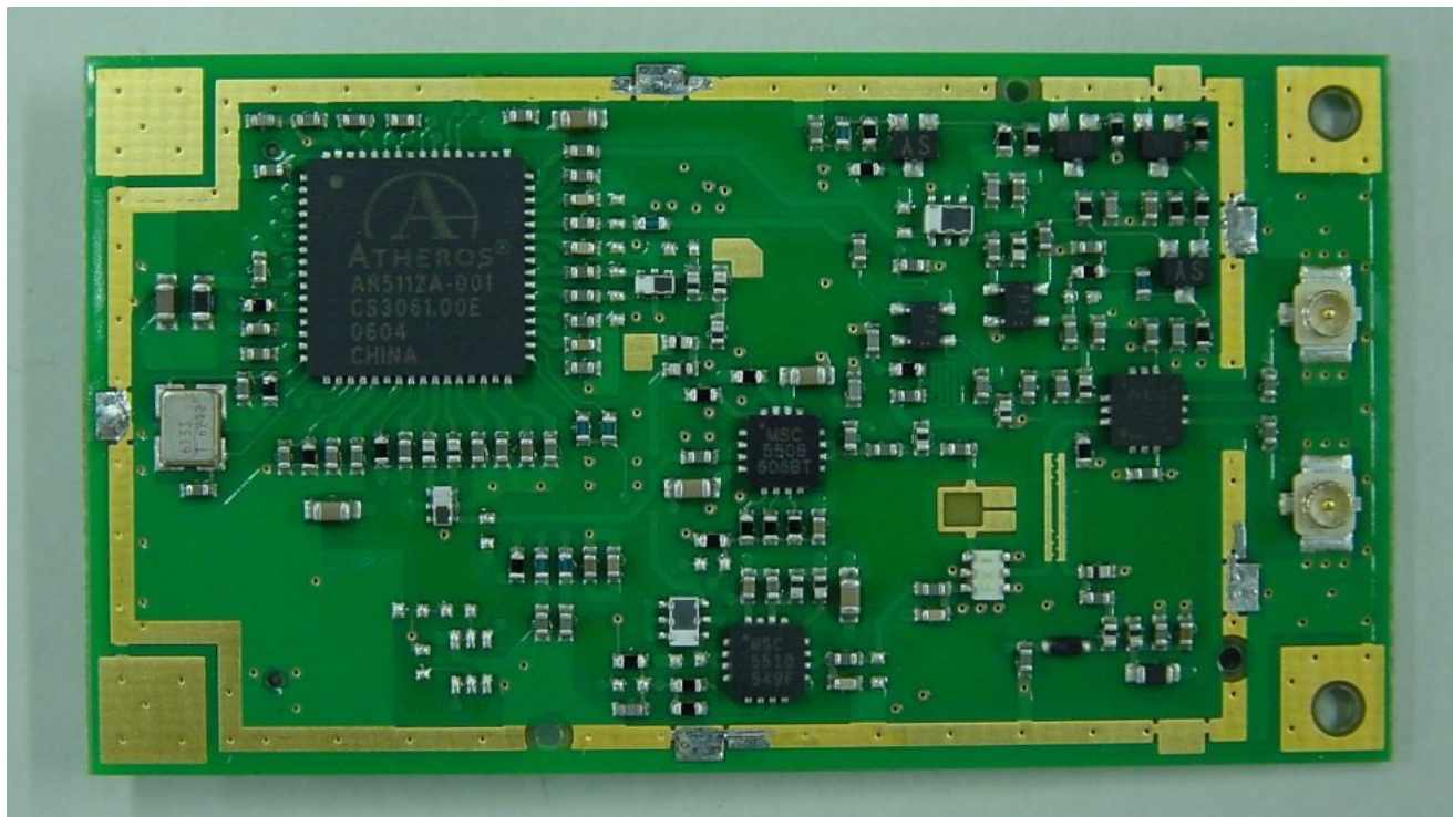
Figure 2 Top View - Without Shield
