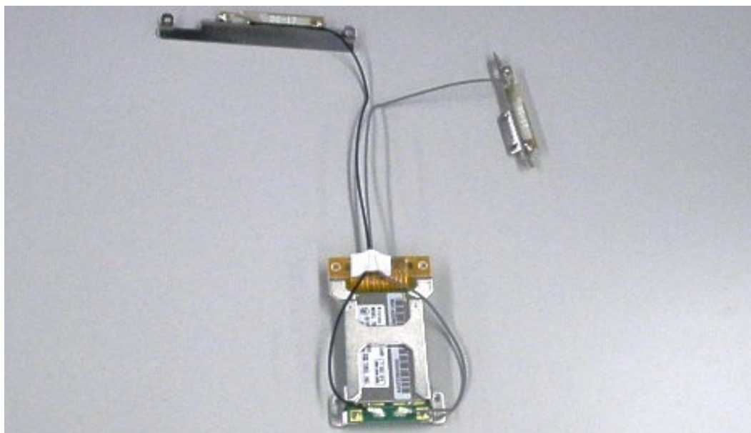
Figure 1 WLAN Card with Antenna & Feedline System Assembly
