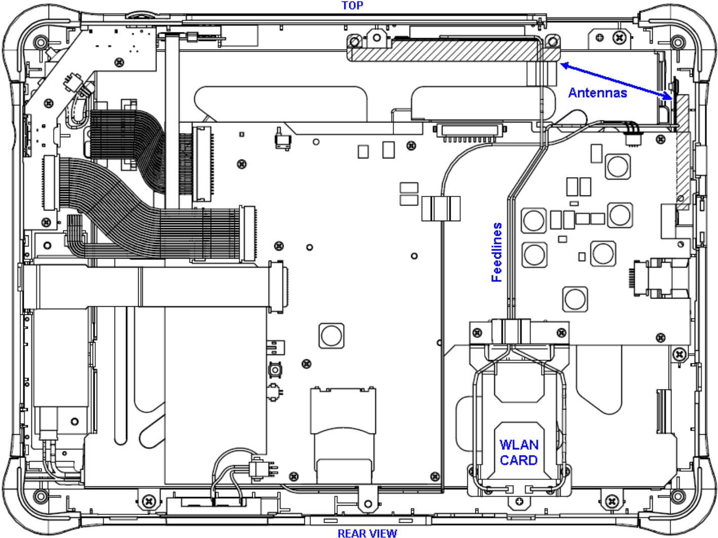
Figure 3 Antenna & Feedline Location Drawing, Rear
