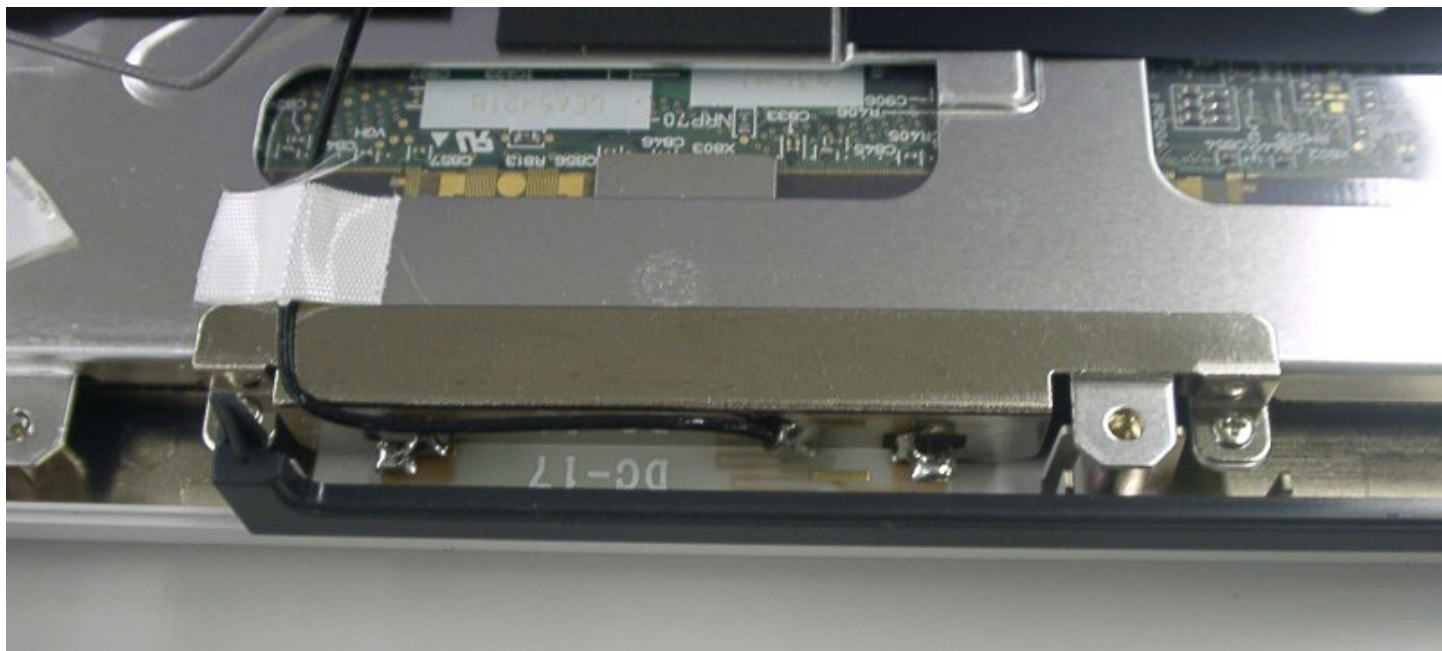
Figure 1 Top Antenna
