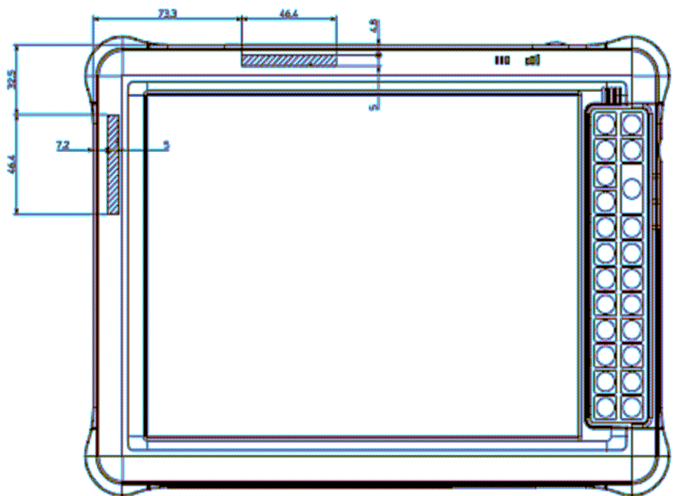
Figure 4 Antenna Locations, Front (shaded rectangles)
