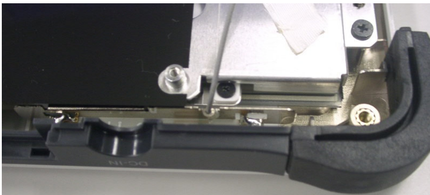
Figure 2 Side Antenna
