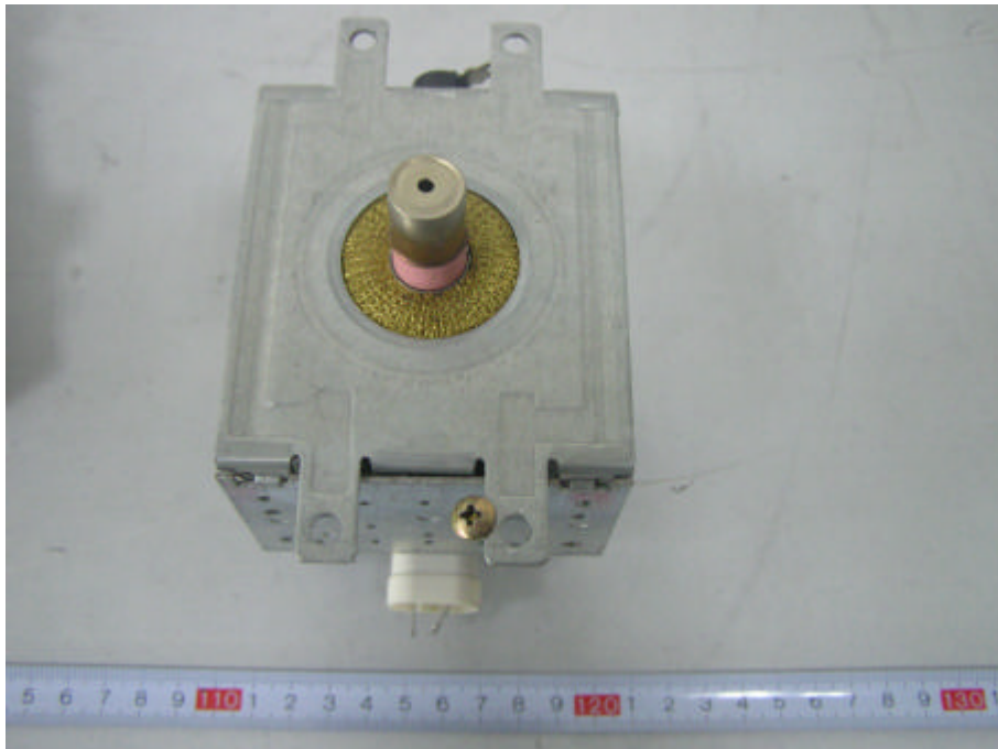
EUT-Magnetron Base view
