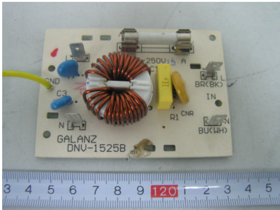
EUT-Power PCB View (1)
