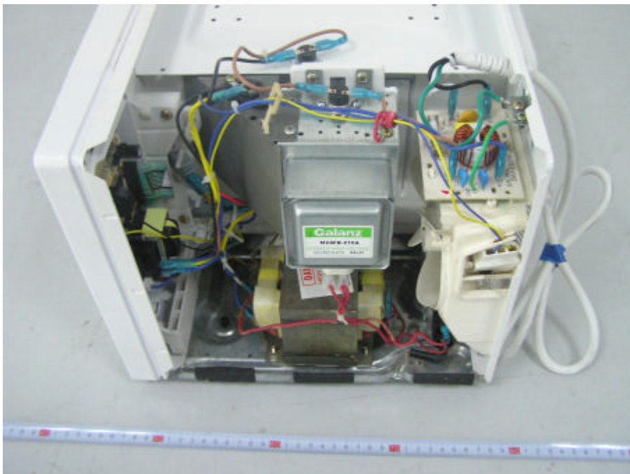
EUT-Inside View (2)
