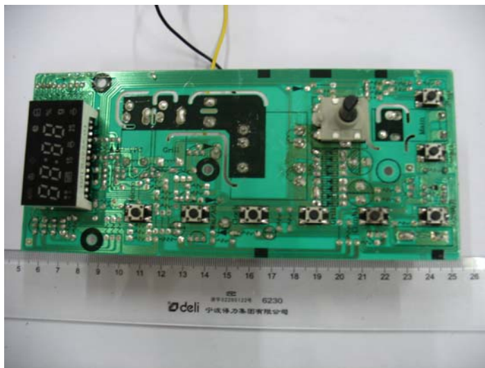
Photo 5 – Back view of main board
