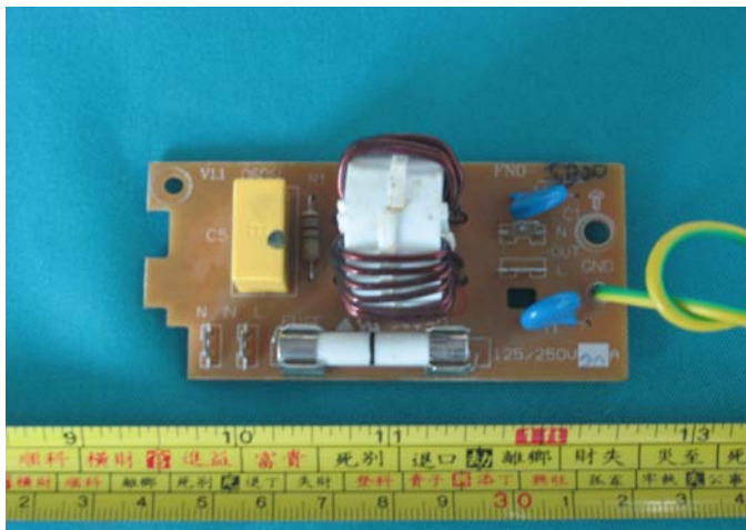
Photo 3 - Back view of AC Power filter board
