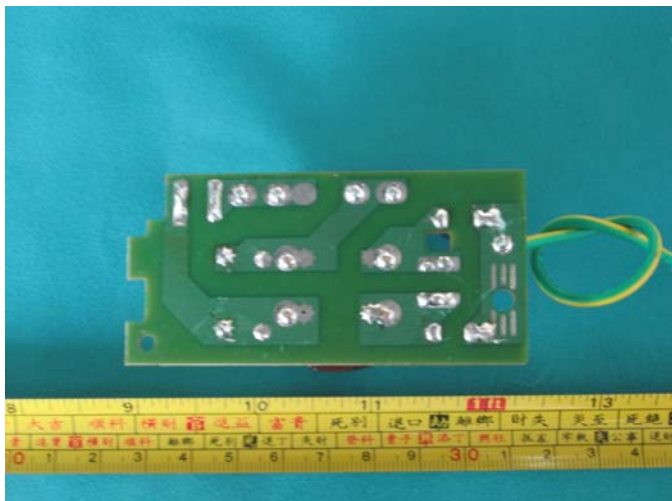
Photo 3 - Back view of AC Power filter board
