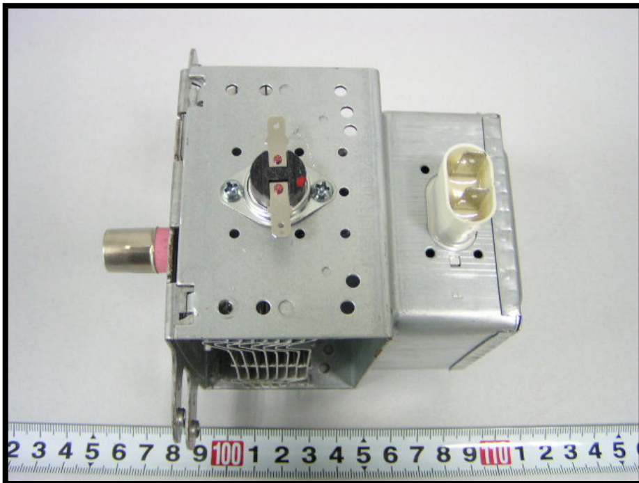
EUT-Magnetron View (1)
