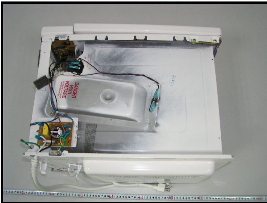
EUT-Inside View (2)
