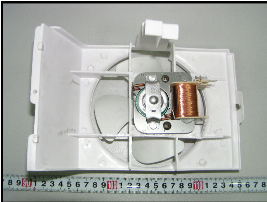
EUT-Fan View (1)
