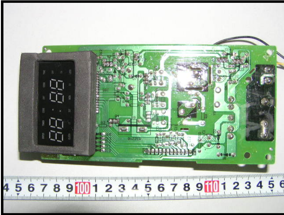
EUT-Fan View (1)
