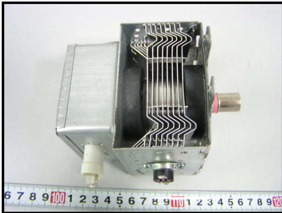
EUT-Magnetron View (3)
