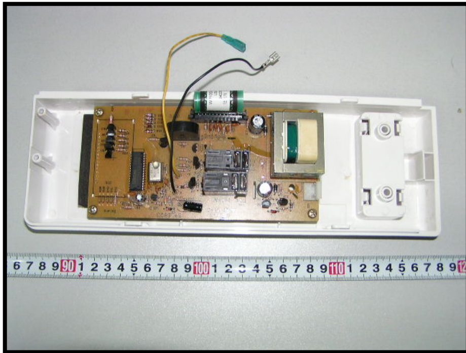
EUT- Control Part inside View (1)
