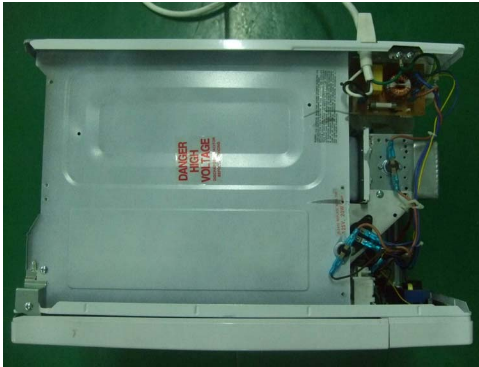
Photo 1- Uncovered view of EUT
