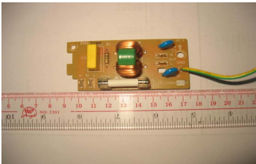
AC power filter board
