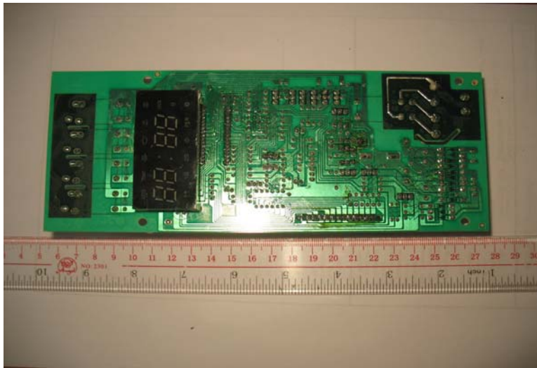
Photo 5 – Back view of main board
