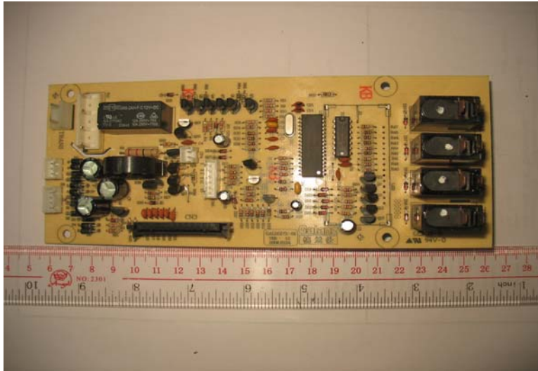
Photo 4 –Front view of Main board
