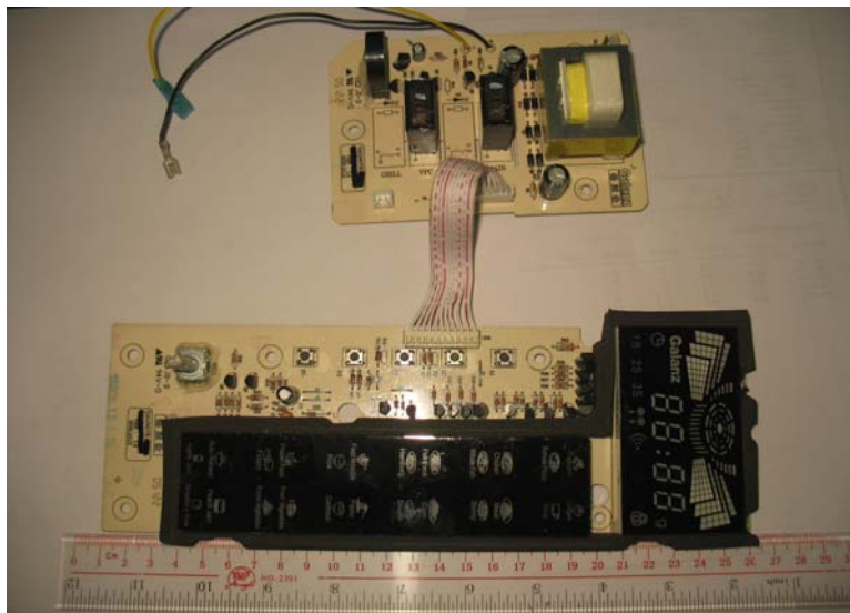
Photo 4 –Front view of Main board
