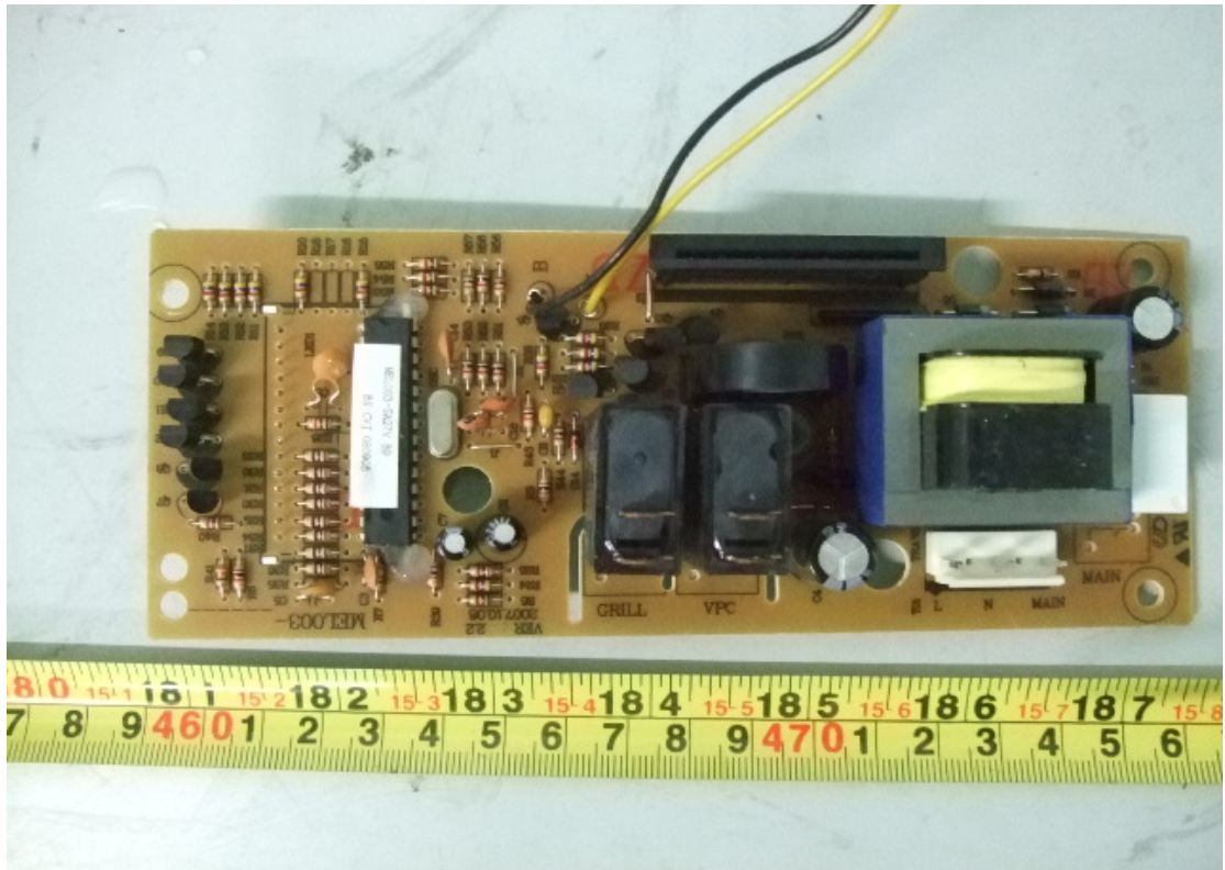
Front view of Main board
