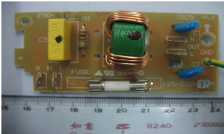
Photo 3 - Back view of AC Power filter board
