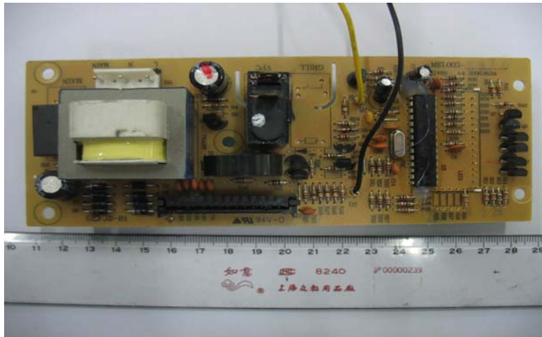
Photo 4 –Front view of Main board
