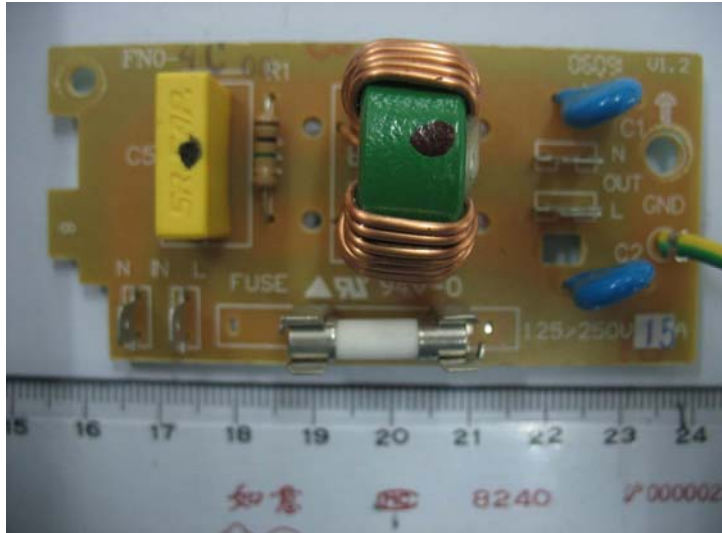
Photo - Front view of AC Power filter board
