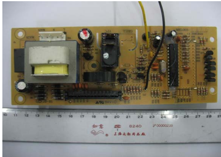
Photo 3 –Front view of Main board
