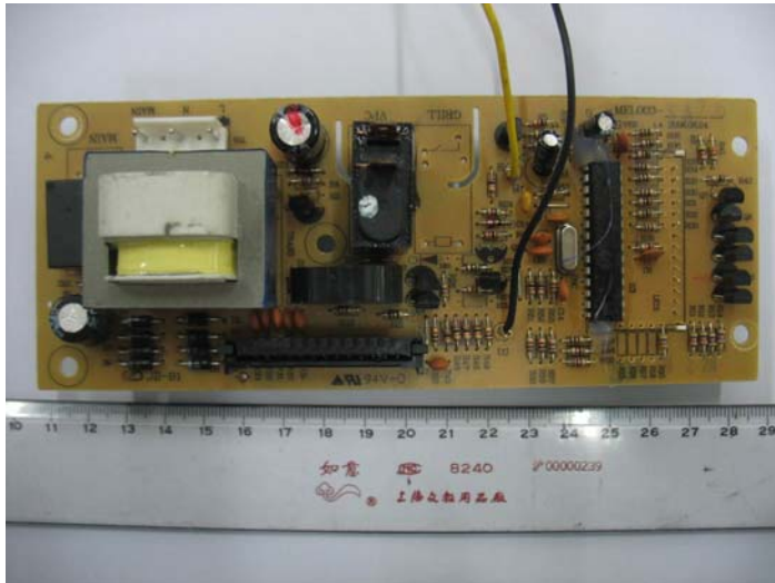
Photo 4 –Front view of Main board
