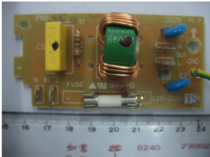
Photo 2- Front view of AC Power filter board
