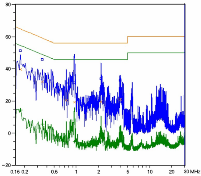
Line N Conducted Emission Graph
