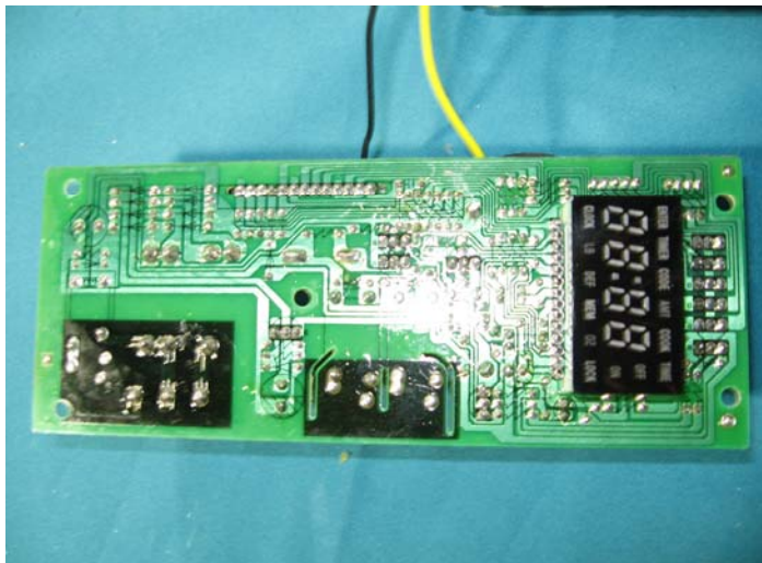
Photo 5 – Back view of main board
