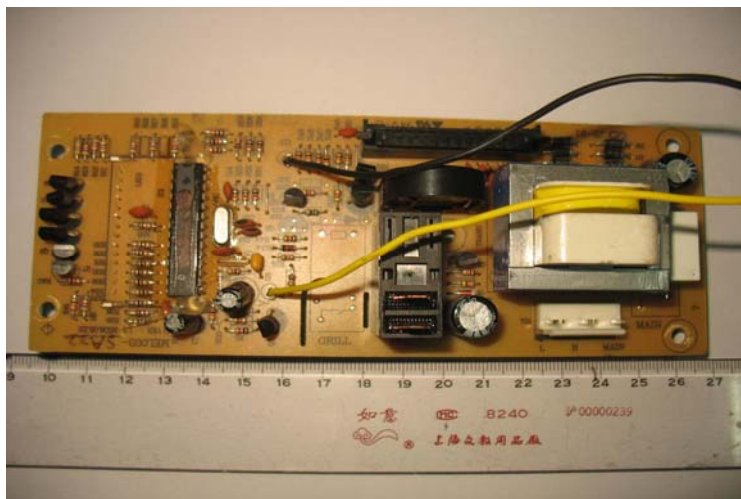
Photo 5 – Back view of main board
