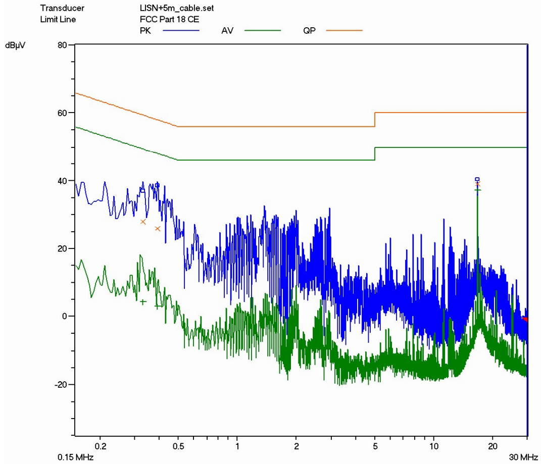
Line N Conducted Emission Graph
