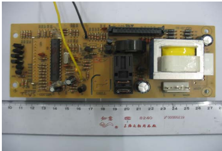
Photo 4 –Front view of Main board
