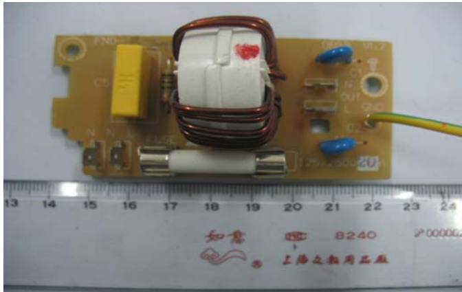
Photo 2- Front view of AC Power filter board
