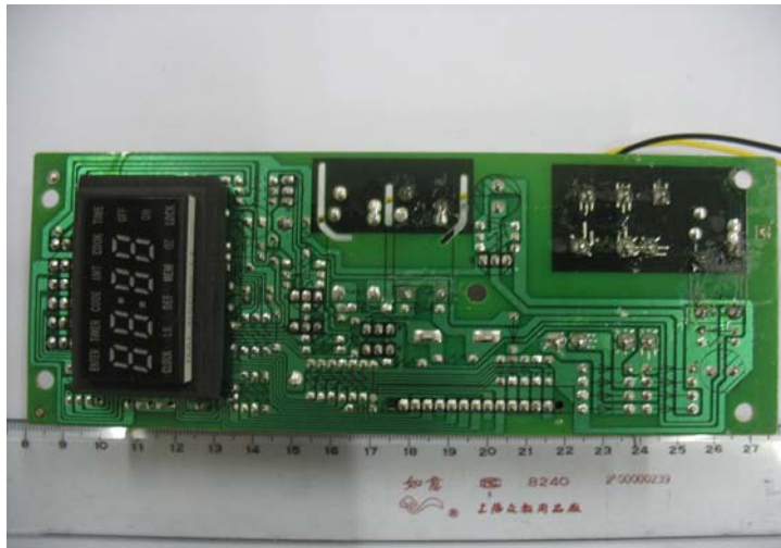
Photo 5 – Back view of main board
