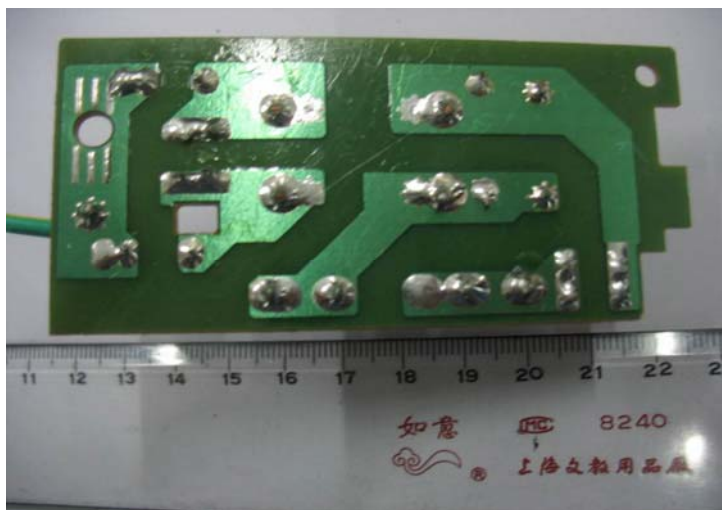
Photo 2 - Back view of AC Power filter board
