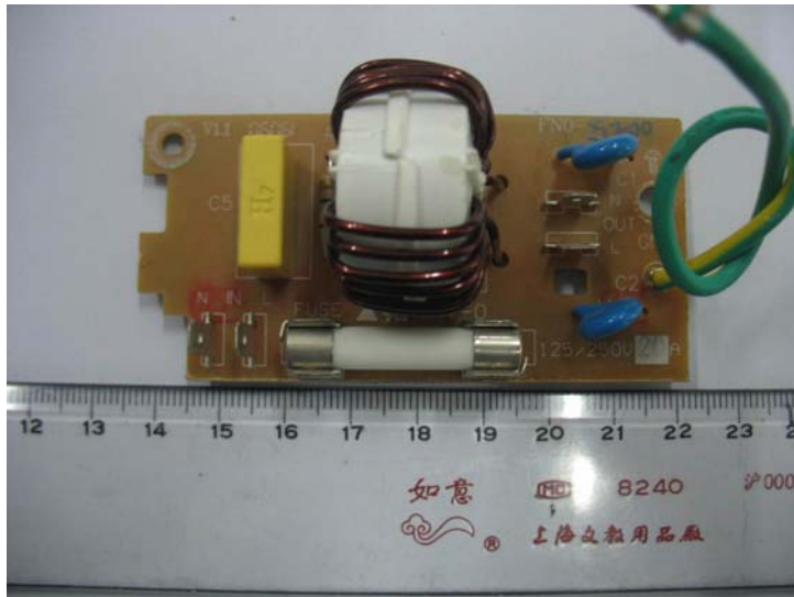
Photo 1- Front view of AC Power filter board
