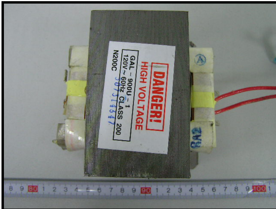
EUT-Transformer View (2)
