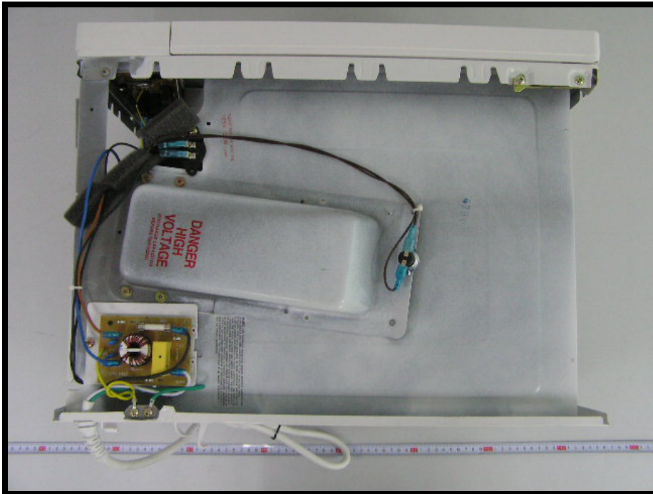
EUT-Inside View
