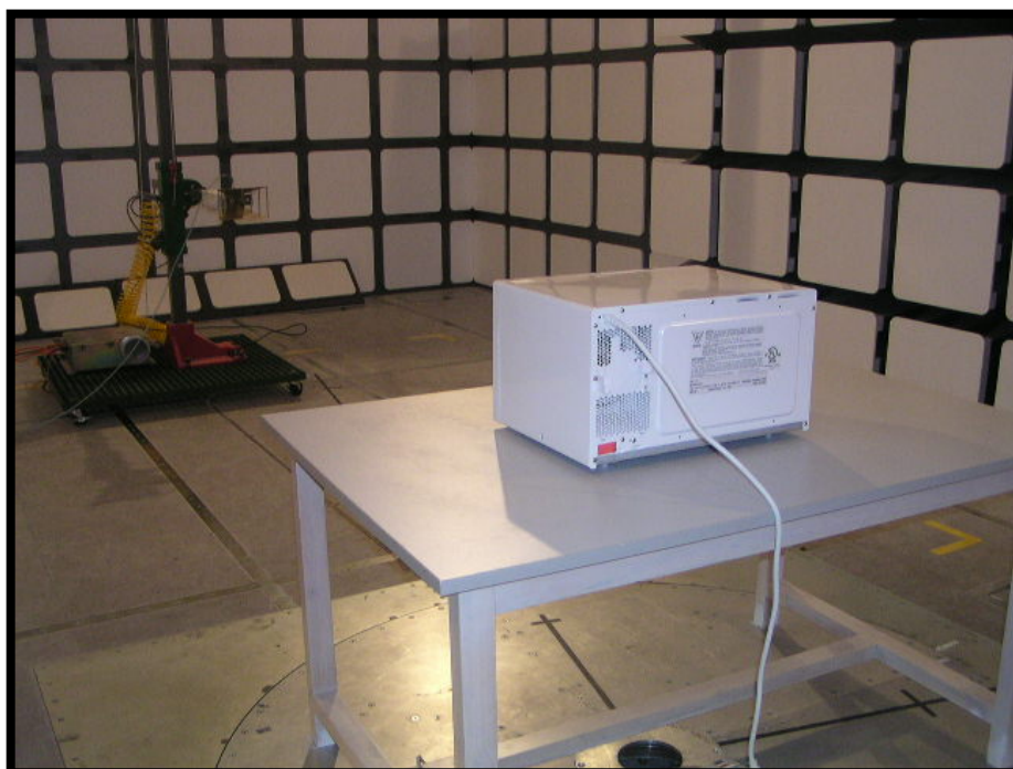
1 GHz-25GHz: Radiated Emission - Rear View
