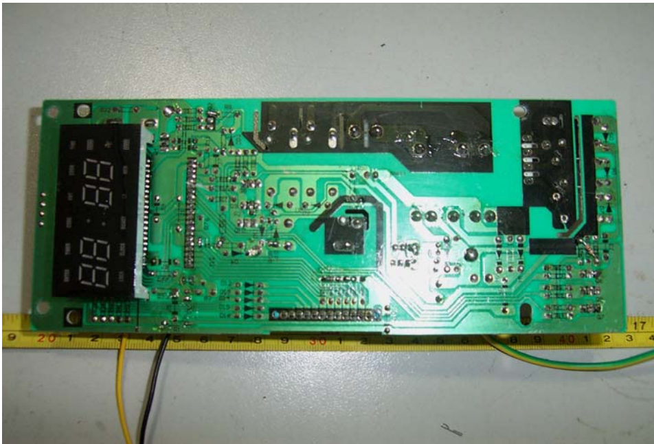
EUT - Solder View (3)
