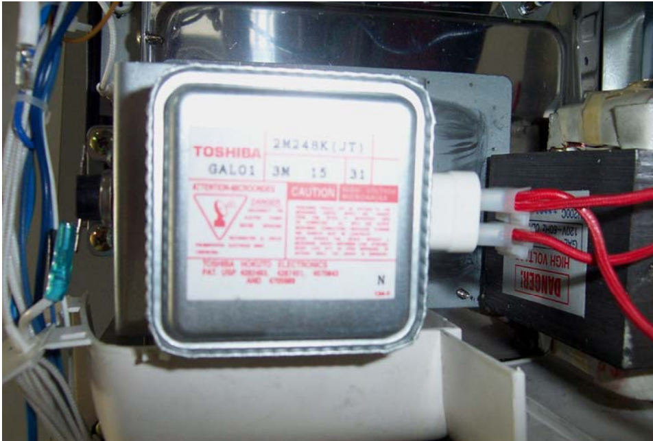
EUT - Inside View (4)
