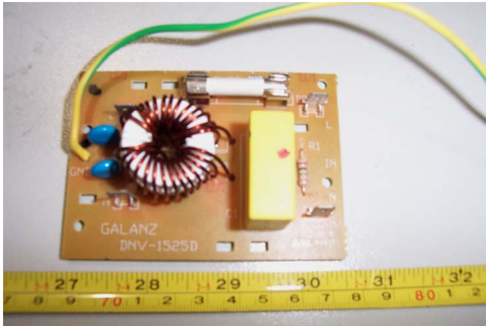
EUT - Component View (1)
