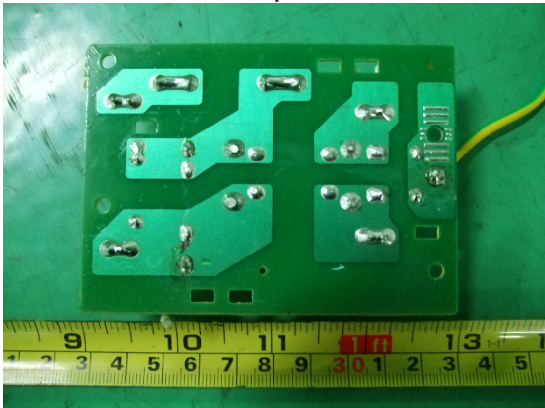
Back View of AC power filter board
