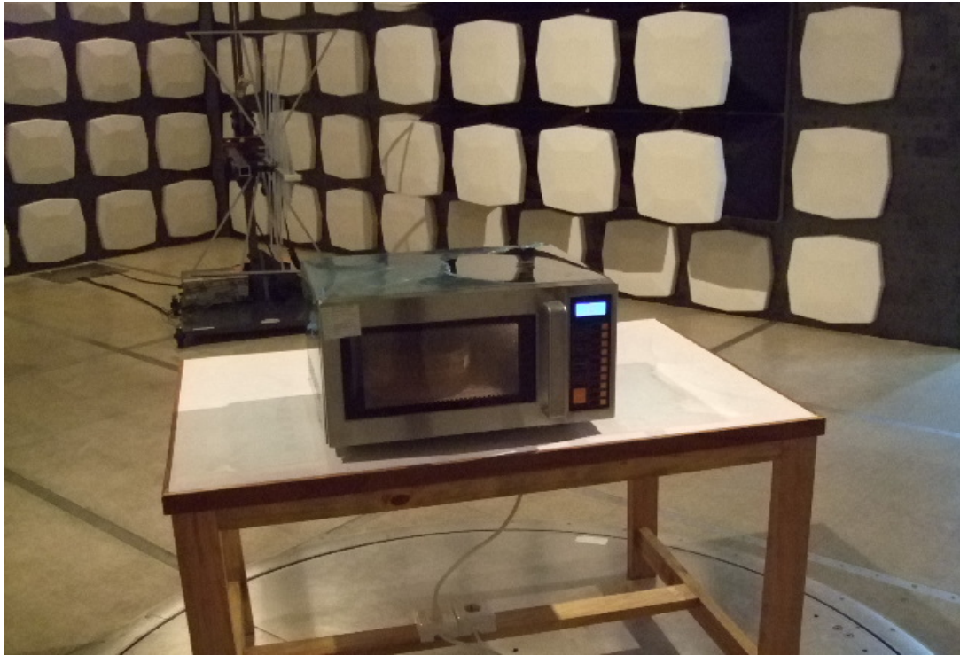
Radiated Emission Test Setup (30-1000MHz)
