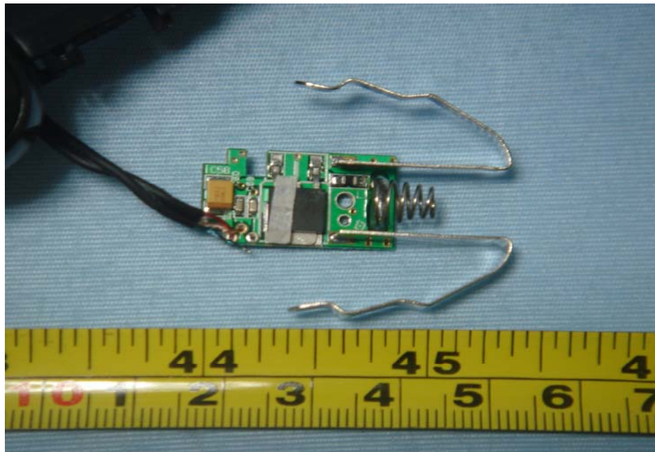
PCB3-Back View
