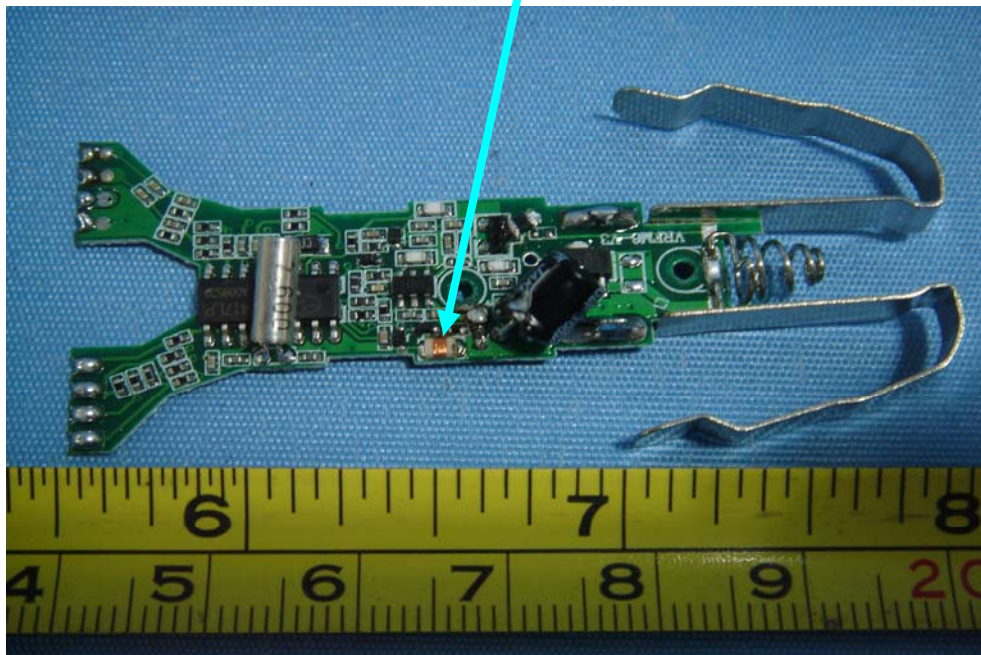
PCB2-Front View
