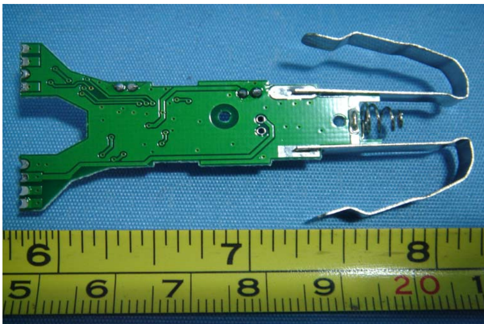
PCB2-Back View
