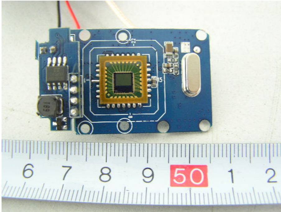
EUT-PCB View (2)
