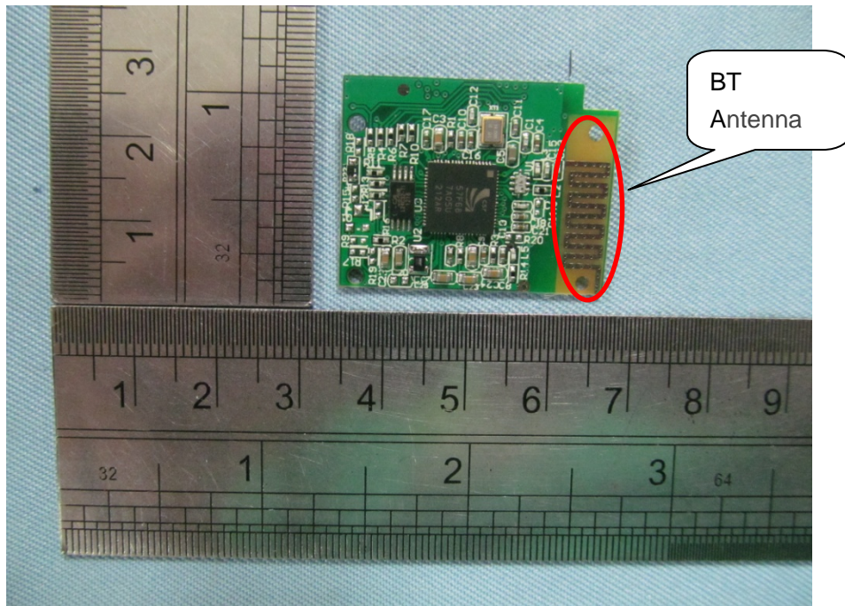
BACK VIEW OF PCB-3
