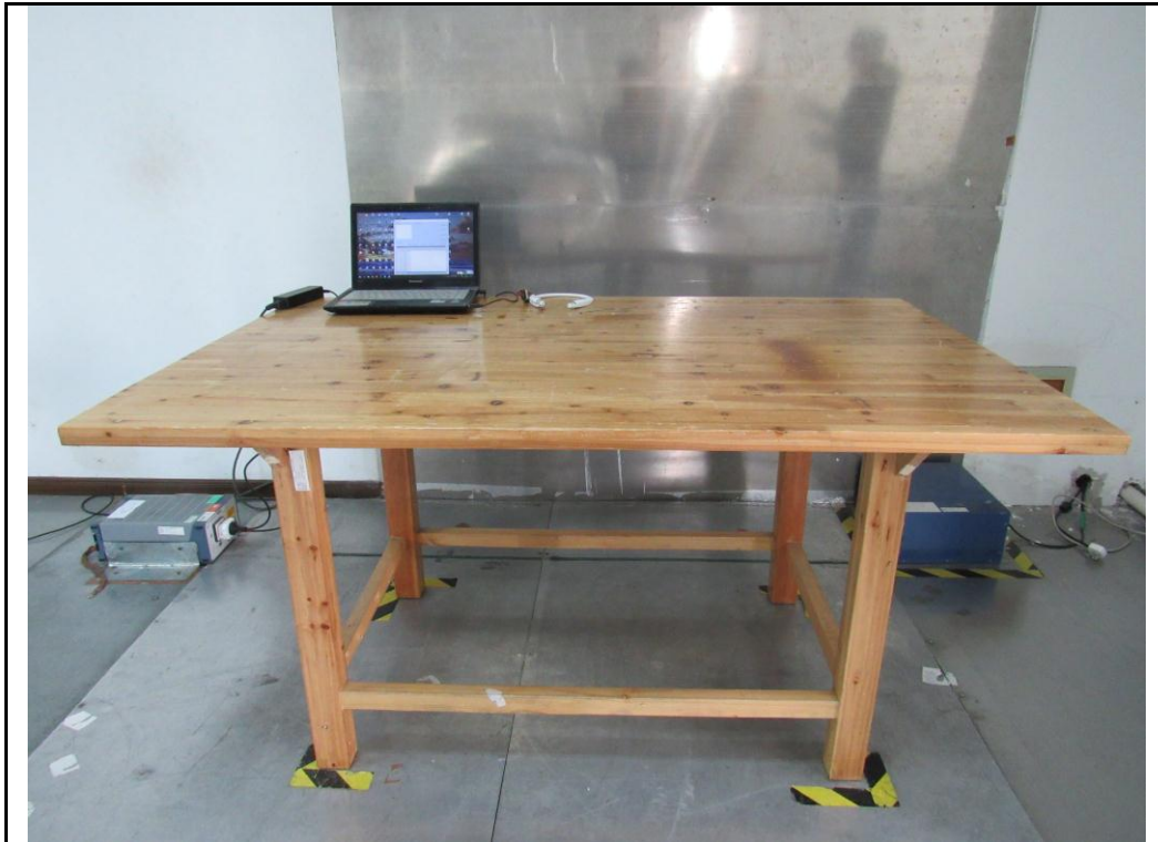
Conducted Emissions Test Setup Front View
