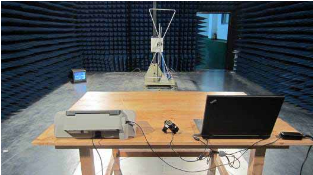
Radiated Emission
