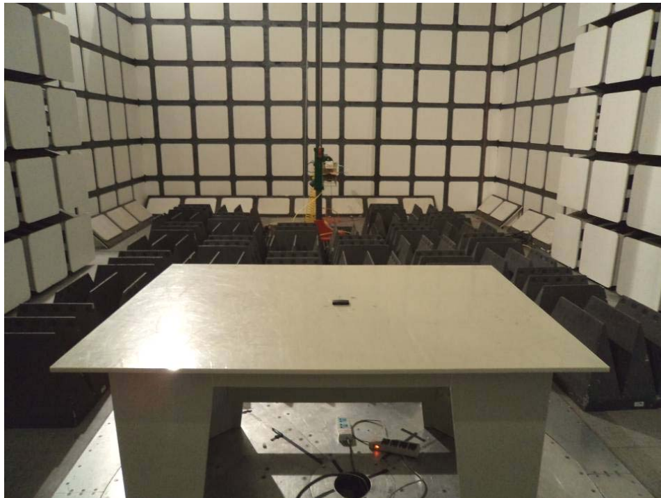
Radiated Emissions Test View (Above 1 GHz)
