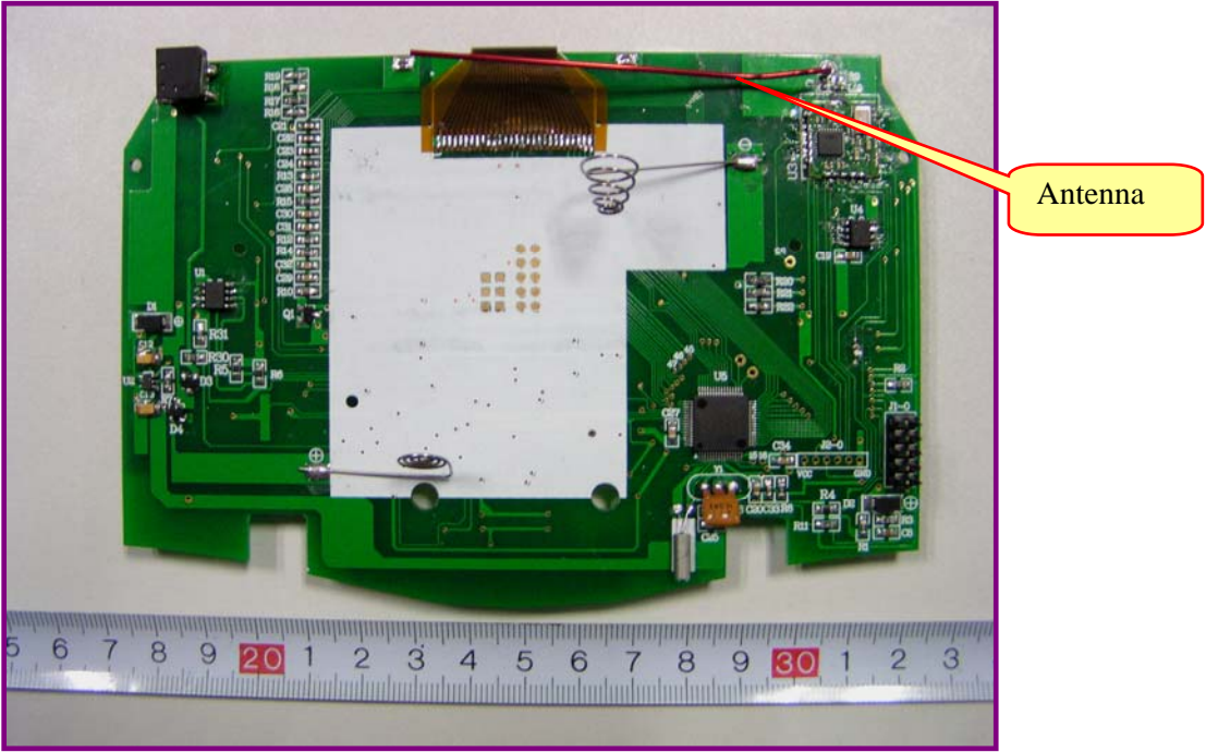
EUT – PCB Bottom View
