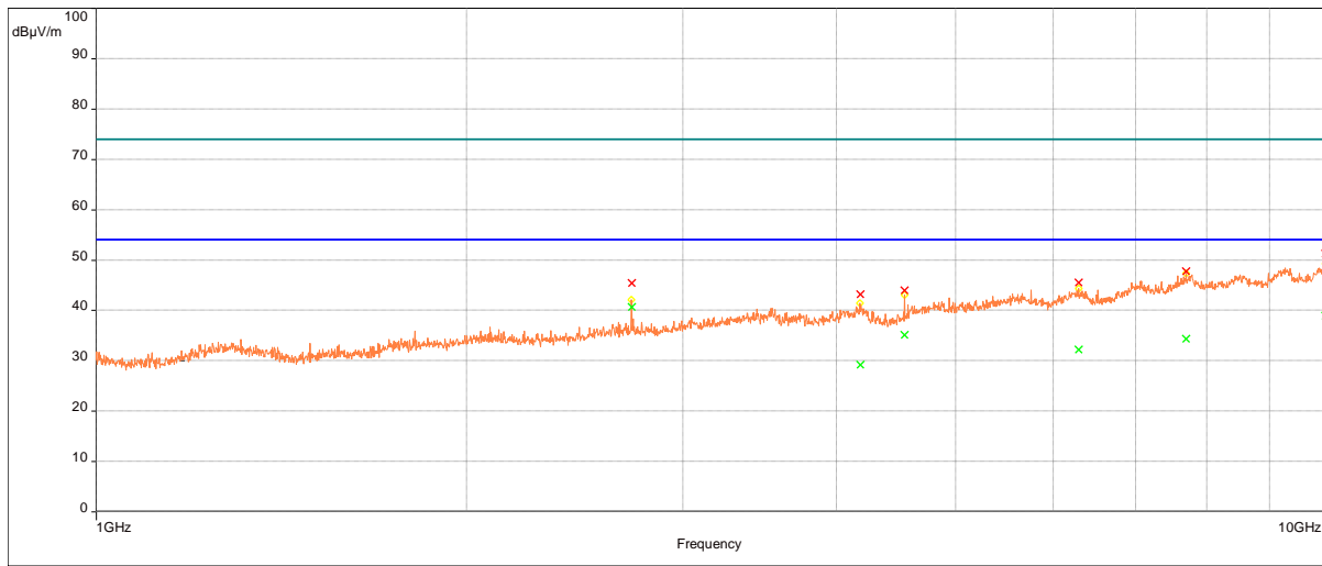
Emissions Graph: RF9617_Z-Axis_RE 1GHz-10GHz -6 power level
