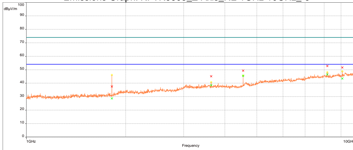
Emissions Graph: RFTR9605_Z-Axis_RE 1GHz-10GHz_-6
