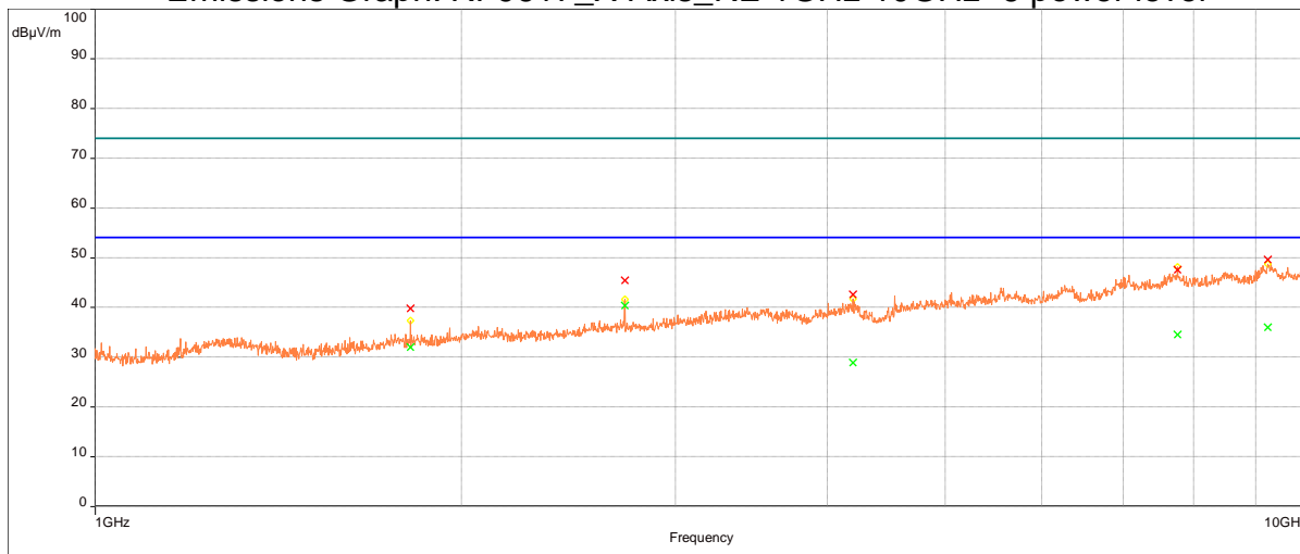
Emissions Graph: RF9617_X-Axis_RE 1GHz-10GHz -6 power level
