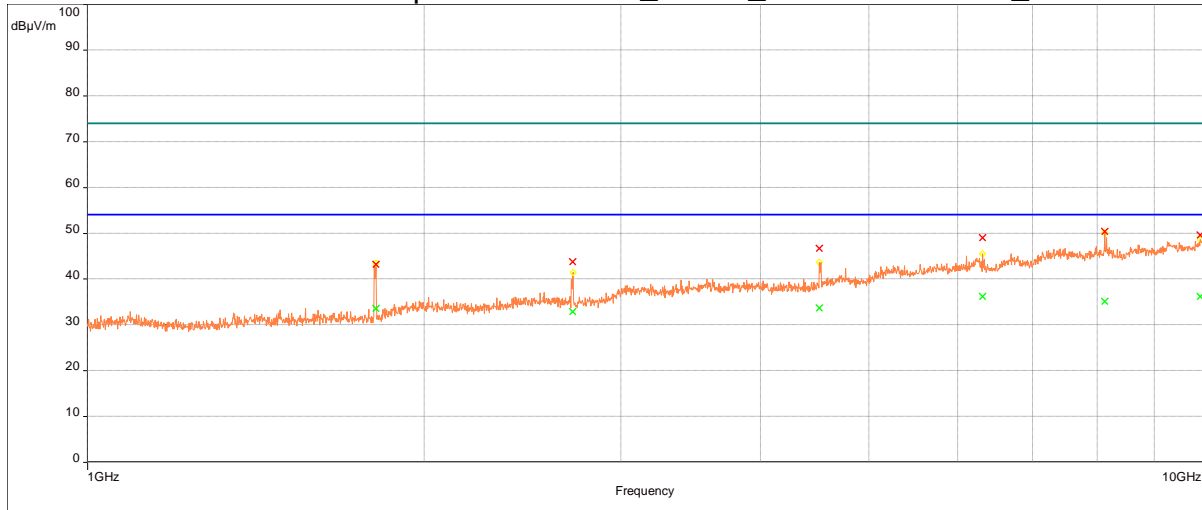
Emissions Graph: 9601 Switch_Z-Axis_RE 1GHz-10GHz_-4
