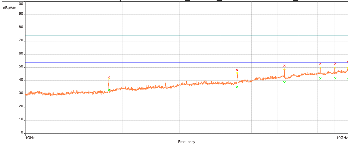
Emissions Graph: 9601 Switch_X-Axis_RE 1GHz-10GHz_-4
