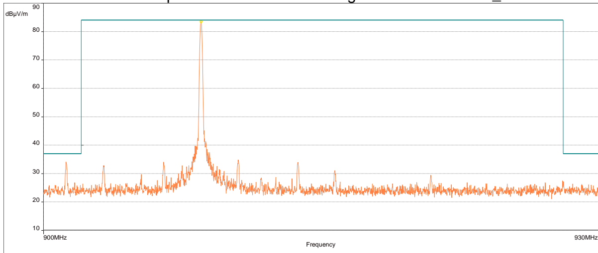
Emissions Graph: RFTR9605 - Band Edge RE 30MHz-1GHz_Z-Axis -2
