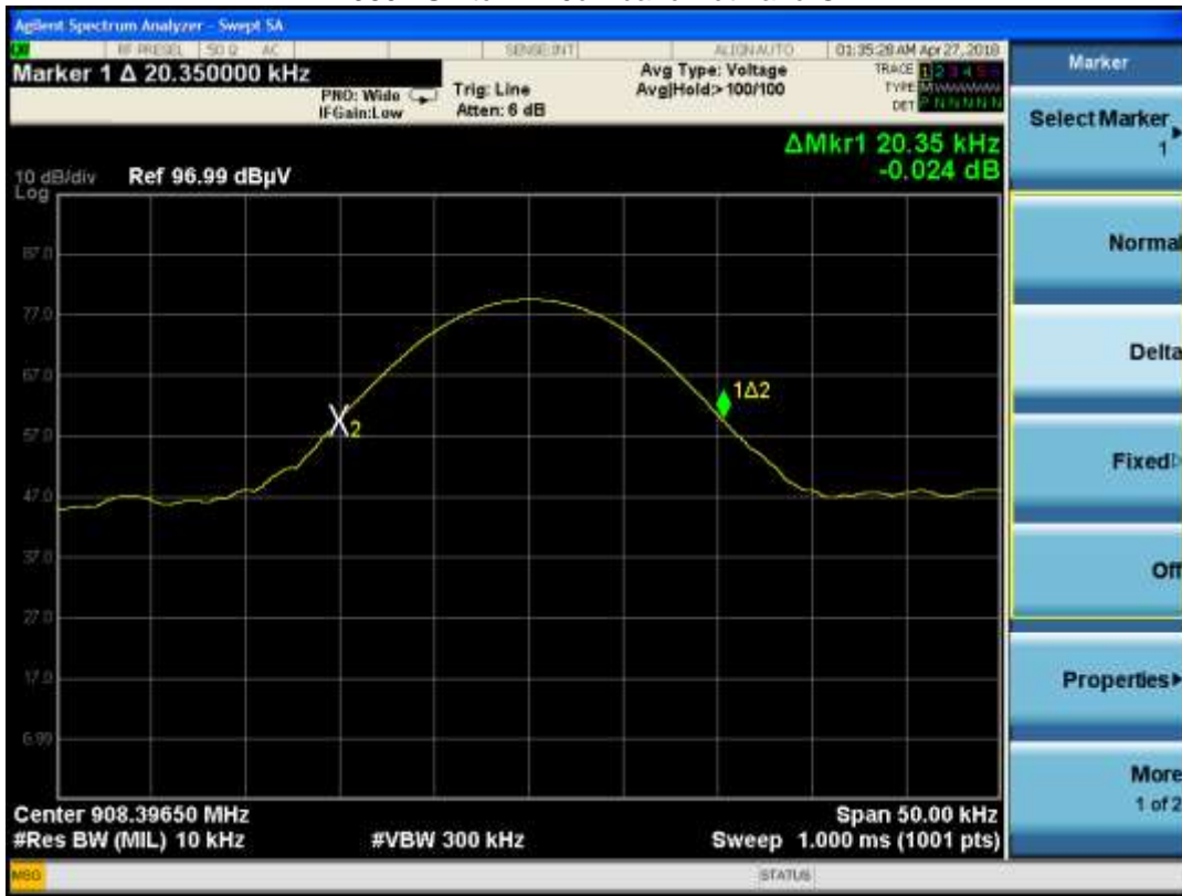
RF9617 Accessory Switch – 20dB bandwidth and OBW
