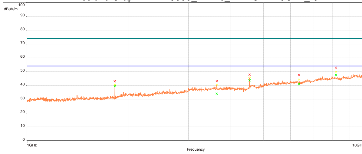
Emissions Graph: RFTR9605_Y-Axis_RE 1GHz-10GHz_-6
