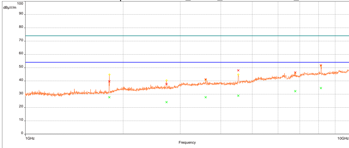
Emissions Graph: 9601 Switch_Y-Axis_RE 1GHz-10GHz_-4
