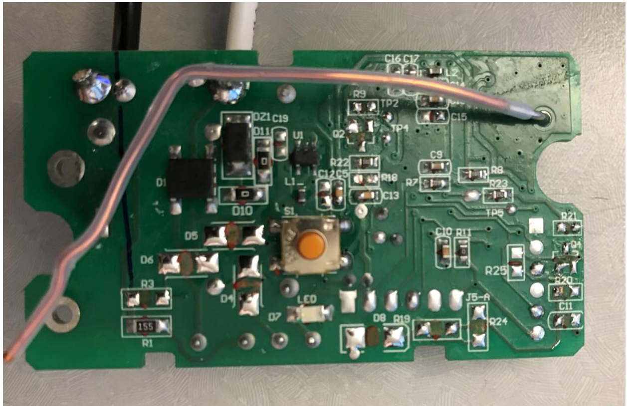
Layout Top view
