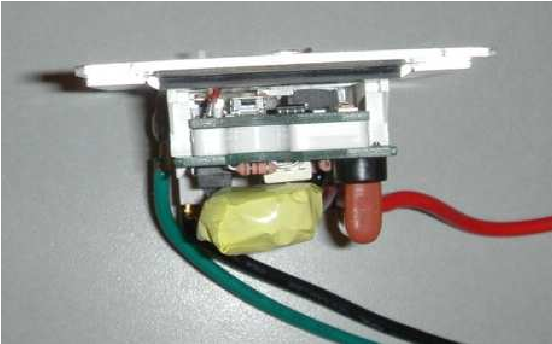
Rf Dimmers Typical Top View.jpg
