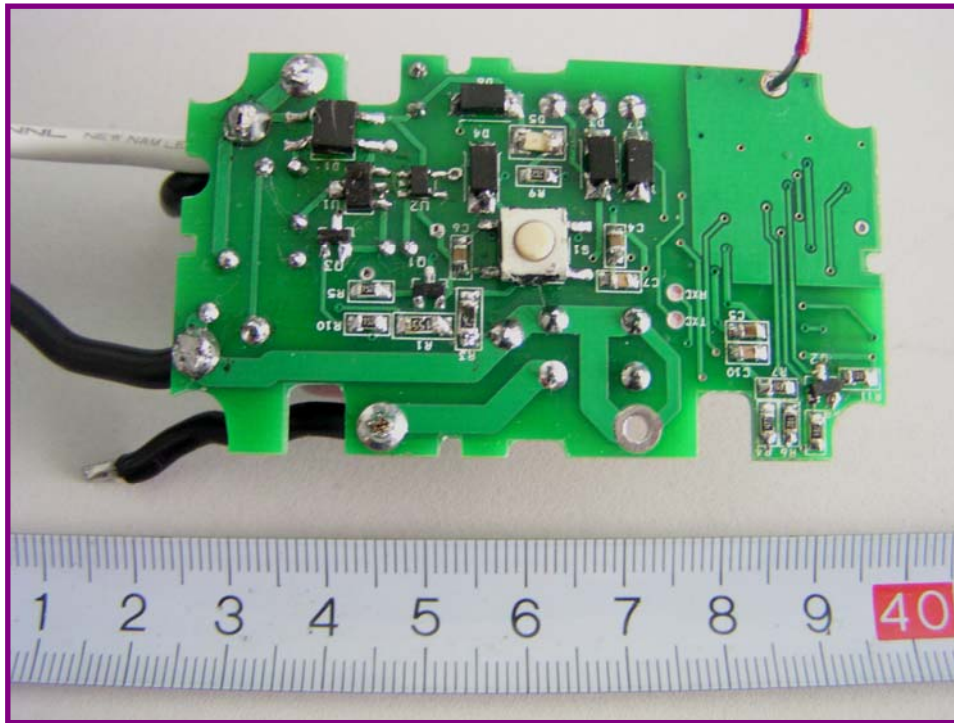
EUT – RF PCB Top View
