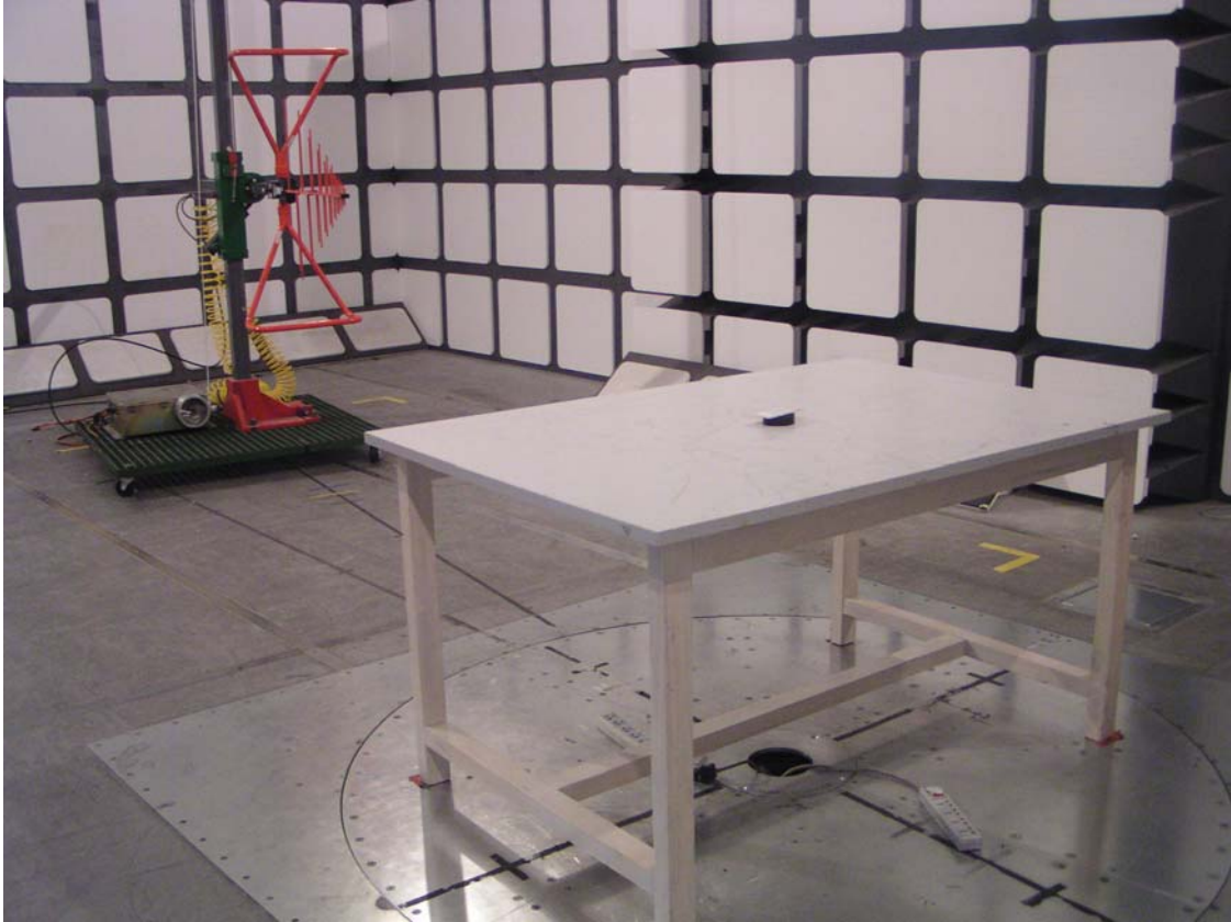
Radiated Emissions - Rear View (30-1000 MHz)
