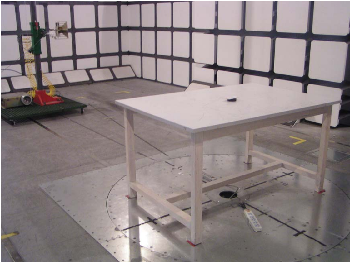
Radiated Emissions - Rear View (Above 1 GHz)
