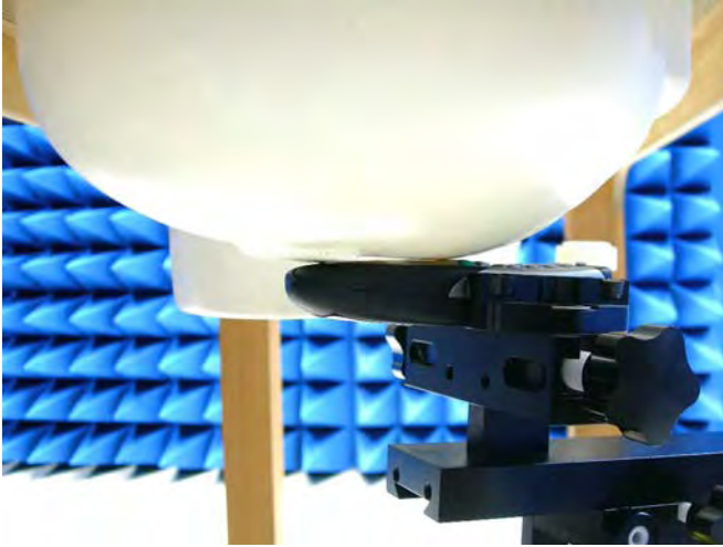
Figure 14. Right Head SAR Test Setup (Cheek)
