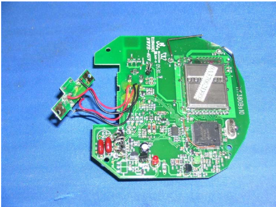
Base Unit Main PCB comp side, LED and Page Key rear side
