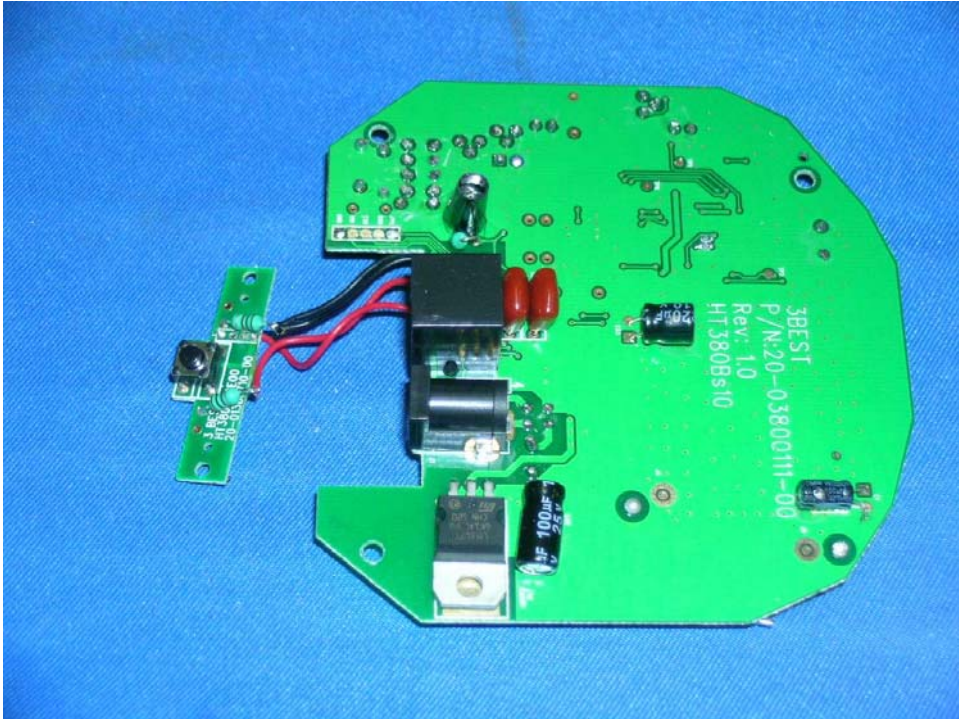
Base Unit Main PCB solder side, LED and Page Key front side
