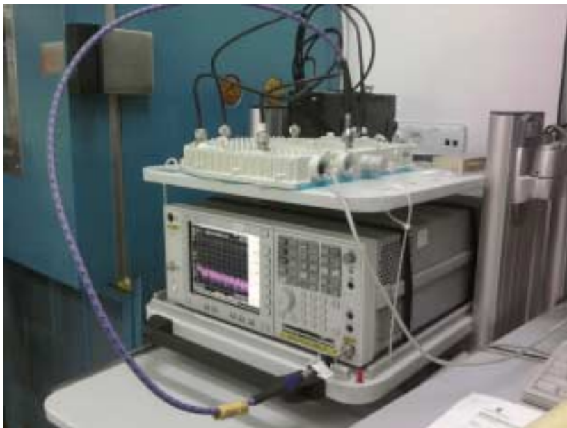
Photograph No.1 Peak output power, occupied bandwidth, emission mask, conducted spurious emissions (single) measurement setup
