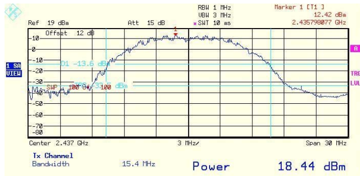
Plot # 146. Output 2 peak power. Middle frequency. 1Mbps rate.
