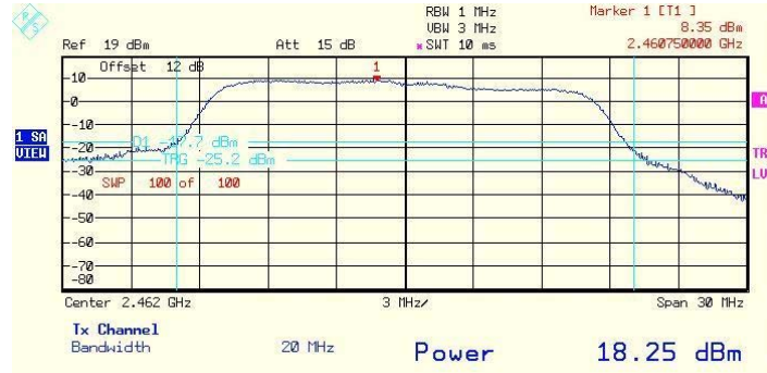
Plot # 149. Output 2 peak power. High frequency. 6Mbps rate.
