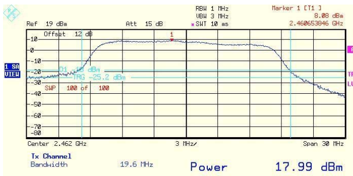
Plot # 161. Output 4 peak power. High frequency. 6Mbps rate.
