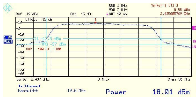
Plot # 153. Output 3 peak power. Middle frequency. 6Mbps rate.
