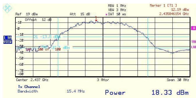
Plot # 152. Output 3 peak power. Middle frequency. 1Mbps rate.
