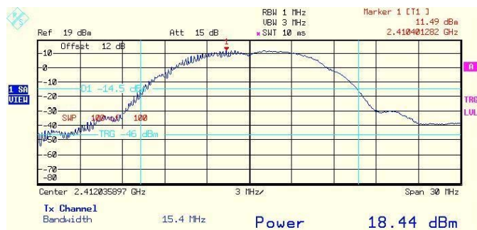
Plot # 144. Output 2 peak power. Lower frequency. 1Mbps rate.
