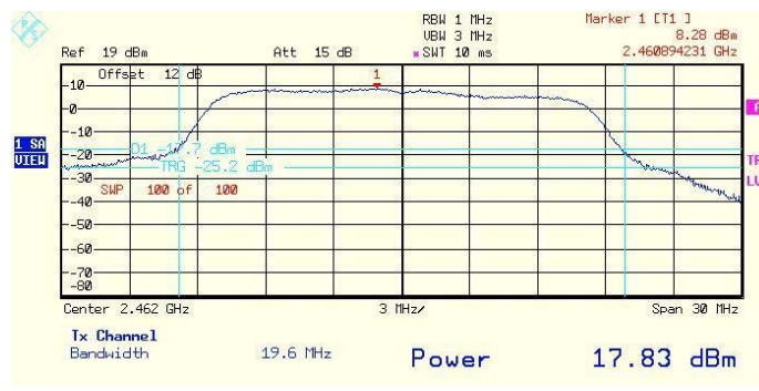
Plot # 155. Output 3 peak power. High frequency. 6Mbps rate.
