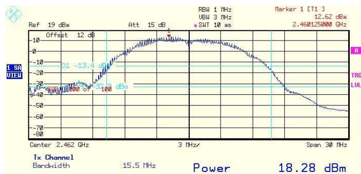
Plot # 148. Output 2 peak power. High frequency. 1Mbps rate.
