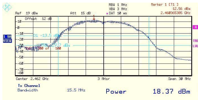
Plot # 160. Output 4 peak power. High frequency. 1Mbps rate.
