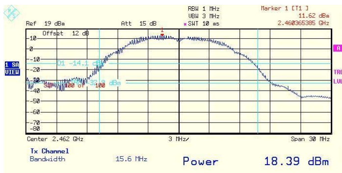
Plot # 154. Output 3 peak power. High frequency. 1Mbps rate.
