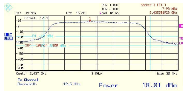
Plot # 159. Output 4 peak power. Middle frequency. 6Mbps rate.
