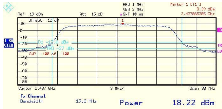
Plot # 147. Output 2 peak power. Middle frequency. 6Mbps rate.
