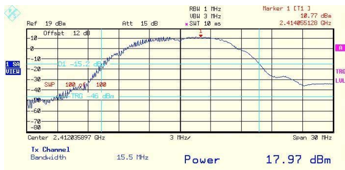
Plot # 156. Output 4 peak power. Lower frequency. 1Mbps rate.
