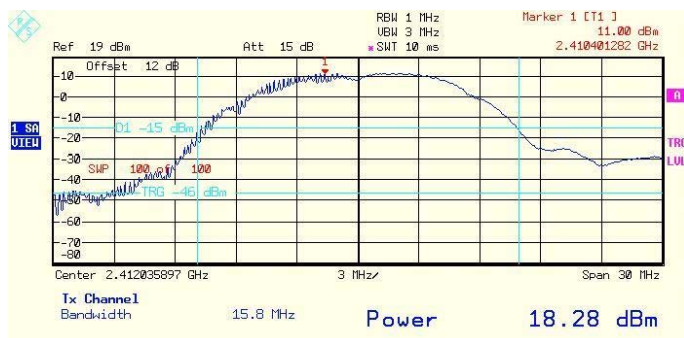
Plot # 150. Output 3 peak power. Lower frequency. 1Mbps rate.
