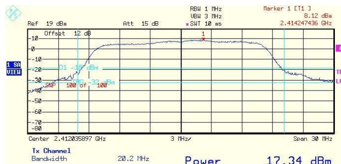
Plot # 145. Output 2 peak power. Lower frequency. 6Mbps rate.
