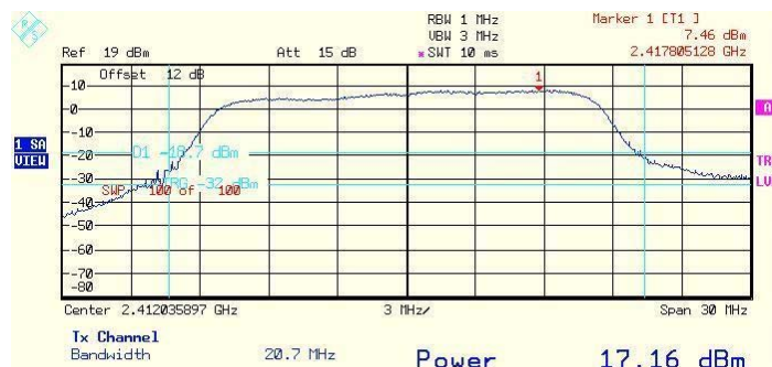
Plot # 157. Output 4 peak power. Lower frequency. 6Mbps rate.
