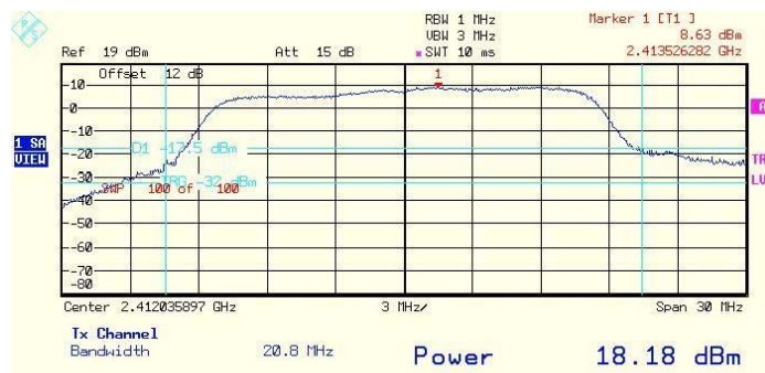
Plot # 151. Output 3 peak power. Lower frequency. 6Mbps rate.
