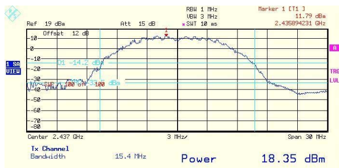
Plot # 158. Output 4 peak power. Middle frequency. 1Mbps rate.
