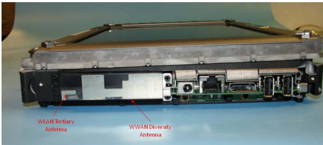
Figure 4 Left View – WWAN Diversity/WLAN Tertiary Antennas
