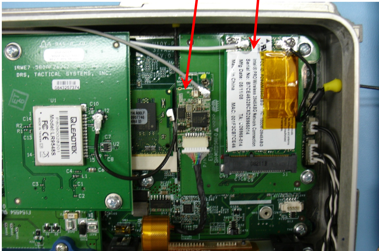
Bottom Assembly
